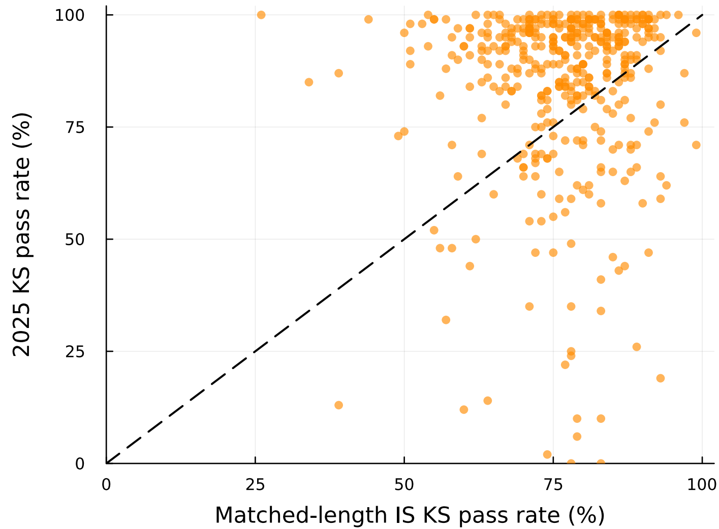
(b) Hybrid: matched IS vs holdout
