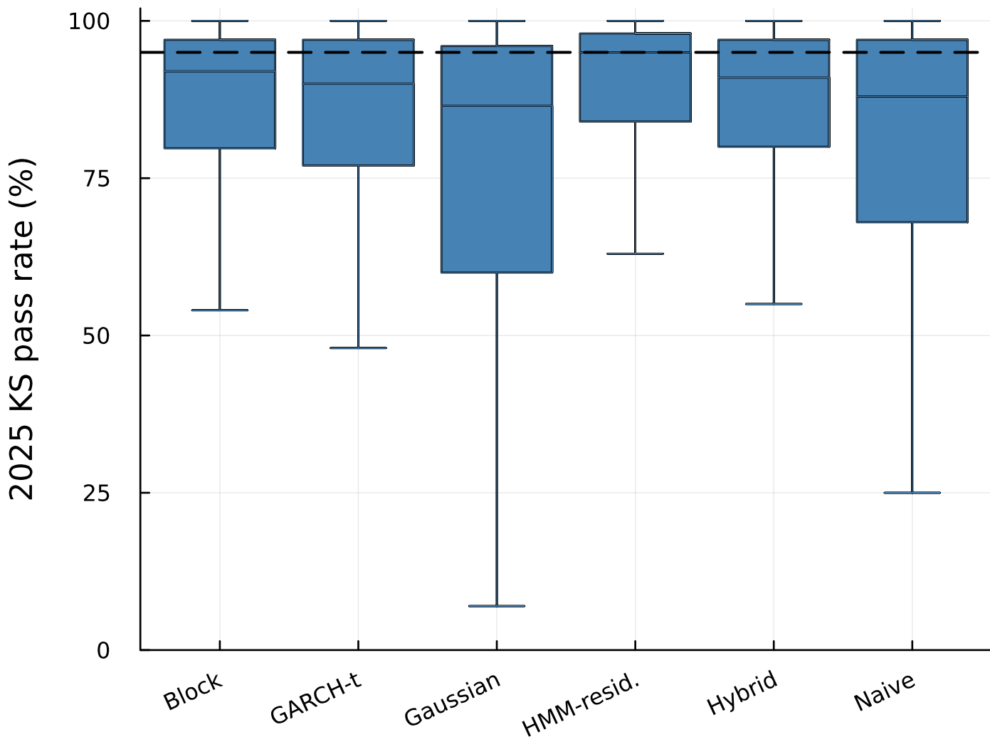
(a) Cross-ticker holdout distribution
