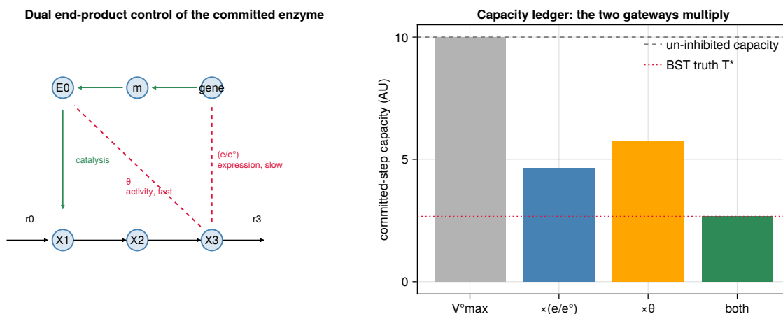
Figure 3: The dual-control feedback worked example. Left: the wiring of the linear chain of Equation (20), in which the end product X_3 closes two negative loops onto the committed step r_0 , repressing transcription of the enzyme’s gene, the slow expression loop acting through (e/e^\circ) , and inhibiting the activity of the enzyme E_0 already present, the fast allosteric loop acting through \theta . Right: the capacity ledger for the committed-step bound of Equation (22). The uninhibited capacity V_{\max, r_0}^\circ = 10 is reduced by the expression gateway alone to 4.64 and by the activity gateway alone to 5.74, and only the two gateways together land on the throughput of the Biochemical Systems Theory truth, T^* \approx 2.66 ; the dashed line marks the uninhibited capacity.
