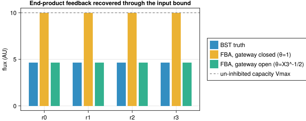
Figure 2: Per-reaction steady-state fluxes for the linear feedback-inhibited pathway of Equation (20). Bars compare the BST S-system truth (throughput T \approx 4.64 ), the flux-balance solution with the regulatory gateway closed ( \theta = 1 , overshooting to the uninhibited capacity of 10 on every reaction), and the flux-balance solution with the gateway open ( \theta = X_3^{-1/2} \approx 0.46 computed from the measured end-product level, recovering the truth). The dashed line marks the uninhibited capacity V_{\max, r_0}^\circ = 10 .
