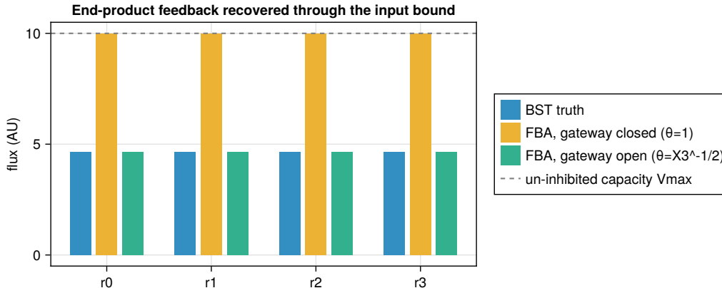
Figure 3: Per-reaction steady-state fluxes for the linear feedback-inhibited pathway of Equation (20). Bars compare the BST S-system truth (throughput T \approx 4.64 ), the flux-balance solution with the regulatory gateway closed ( \theta = 1 , overshooting to the uninhibited capacity of 10 on every reaction), and the flux-balance solution with the gateway open ( \theta = X_3^{-1/2} \approx 0.46 computed from the measured end-product level, recovering the truth). The dashed line marks the uninhibited capacity V_{\max, r_0}^\circ = 10 .
