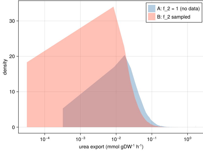
Figure 2: Saturation-gateway sensitivity for urea export. Configuration A (blue) samples the four saturation factors that Park and coworkers [15] constrain and holds f_2 = 1 at the argininosuccinate lyase bottleneck, whose substrate is unmeasured, giving a median urea export of 0.029 \text{ mmol gDW}^{-1} \text{ h}^{-1} . Configuration B (red) imputes f_2 from a physiological argininosuccinate concentration and a BRENDA Michaelis constant and samples it as well, pulling the median down to 0.014 \text{ mmol gDW}^{-1} \text{ h}^{-1} and widening the band toward zero. The horizontal axis is logarithmic.
