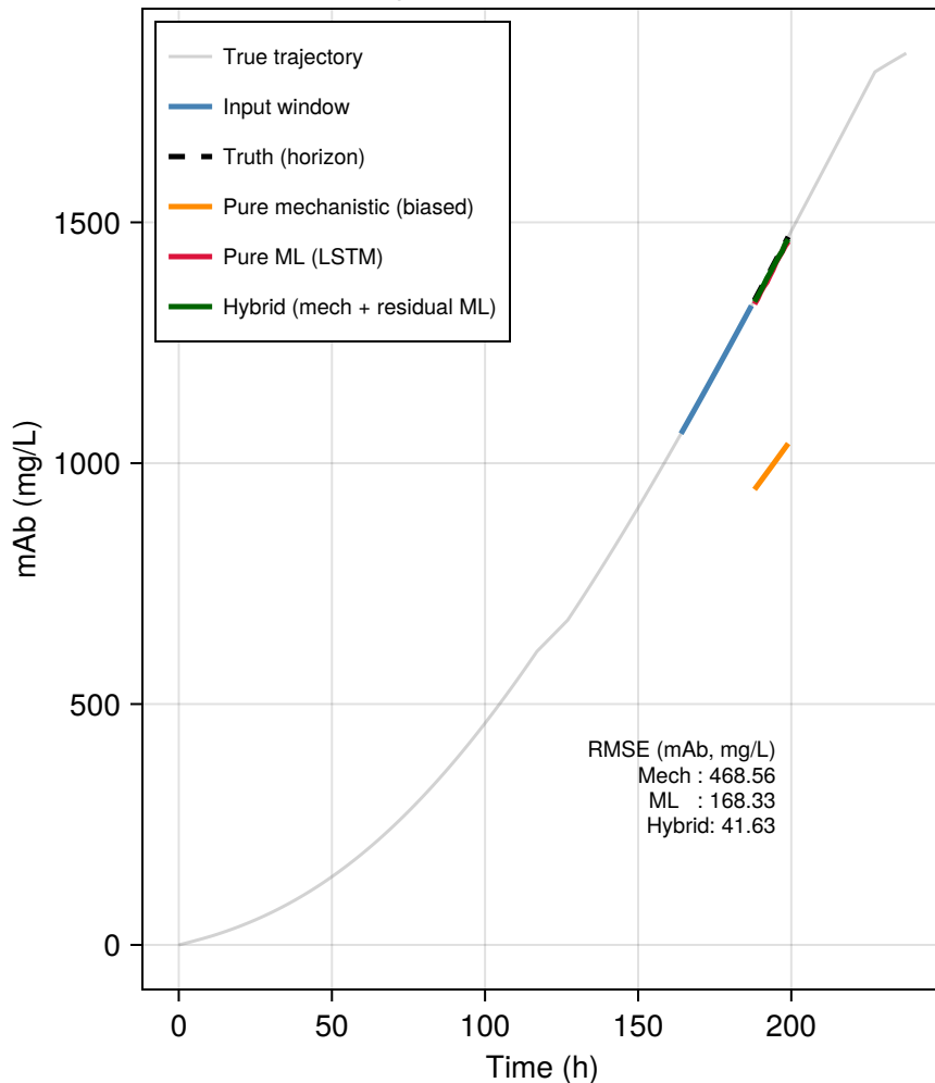
CHO Hybrid Model: mAb Forecast
