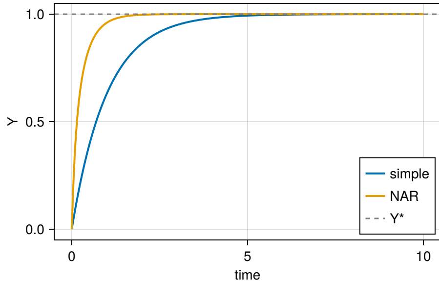
(A) Negative autoregulation
