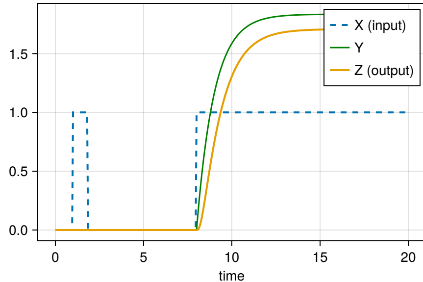
(B) C1-FFL — persistence detector
