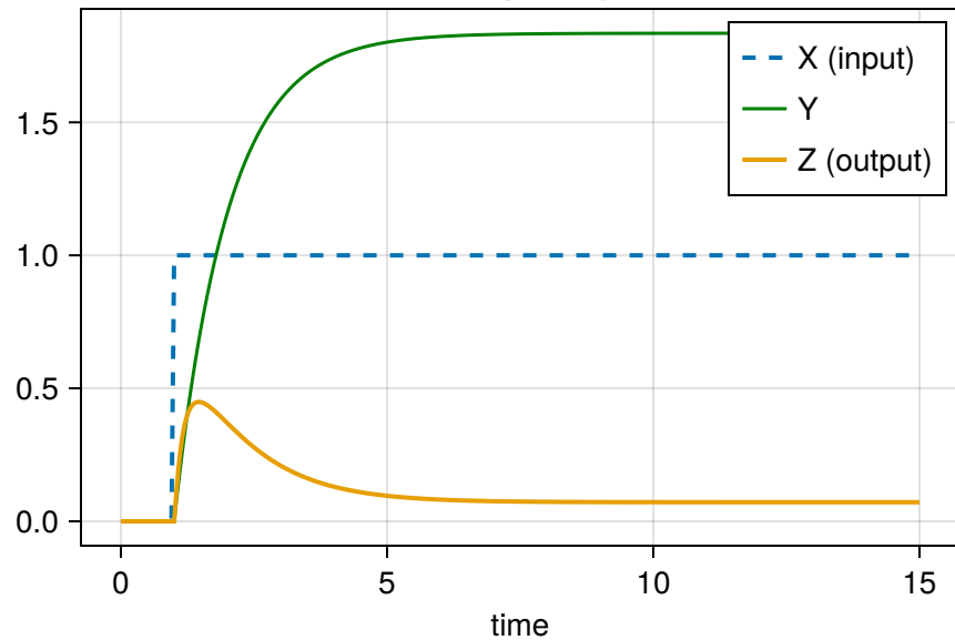
(C) I1-FFL — pulse generator
