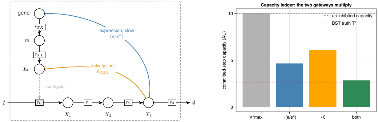
Figure 3: The dual-control feedback worked example. Left: the wiring of the linear chain of Equation (18) inside the dashed cell boundary, with the metabolic backbone r_0 through r_3 along the bottom and the transcription and translation cascade that builds the committed enzyme E_0 down the left. The end product X_3 closes two repressing loops, drawn as blunt-ended arrows, that set the capacity of the committed step r_0 : the slow expression loop onto the enzyme’s gene, acting through (e/e^\circ) and drawn in blue, and the fast allosteric loop onto the enzyme E_0 already present, acting through \theta_{\text{FBA}} and drawn in orange, the two colors matching the corresponding capacity markdowns at right. Right: the capacity ledger for the committed-step bound of Equation (20). The uninhibited capacity V_{\text{max},r_0}^\circ = 10 is reduced by the expression gateway alone to 4.64 (blue) and by the activity gateway alone to 6.10 (orange), and only the two gateways together approach the throughput of the Biochemical Systems Theory truth, T^* \approx 2.66 , landing at 2.83; the dashed line marks the uninhibited capacity.
