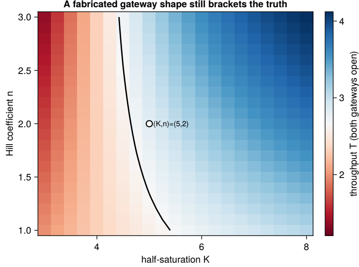
Figure 4: Robustness of the dual-gateway recovery to the fabricated activity-gateway shape. The committed-step throughput with both gateways open, \hat{v}_{r_0} = V_{\max, r_0}^{\circ} (e/e^{\circ}) \theta_{\text{FBA}} , is shown as the made-up Hill shape \theta_{\text{FBA}} = K^n / (K^n + X_3^n) of Equation (21) is swept over its half-saturation K and cooperativity n , with the measured X_3 , the expression ratio, and every other bound held. The color scale diverges about the Biochemical Systems Theory truth T^* \approx 2.66 , red below and blue above, and the black contour is the locus where the reconstruction equals the truth exactly; the recovered throughput runs from about 1.4 to about 4.1, so the truth lies inside the reachable band. The marked point is the shape the rest of the construction carries, (K, n) = (5, 2) , returning 2.83. Neither single gateway reaches the truth for any shape in the window: opened alone the expression gateway holds the step at 4.64 and the activity gateway stays above about 2.97, so only the two together bracket T^* .
