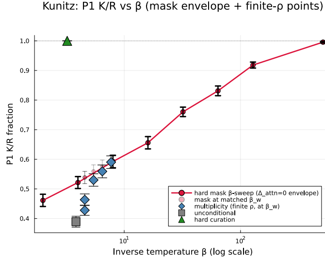
Figure 4: Recovery is set by retrieval sharpness and conditioning strength, both acting through the decode gap. P1 K/R fraction for the Kunitz designated subset versus inverse temperature \beta (log scale) under the hard attention mask ( b = -\infty on background patterns; red curve, 30 chains per point, error bars are standard error across chains). The mask is the \Delta_{\text{attn}} = 0 envelope: recovery climbs monotonically from 0.46 at \beta = 2 to 1.00 at \beta = 512 with no plateau. The finite- \rho multiplicity conditions (blue diamonds, each at its own \beta^*(\mathbf{r}) ) sit below this envelope at matched \beta : hard masking recovers more phenotype than soft weighting by 0.111 (SE 0.027) at f_{\text{eff}} = 0.5 , contracting into the noise as \rho \rightarrow \infty (0.002, SE 0.030, at f_{\text{eff}} = 0.99 ); faint red points show the mask run at each matched \beta . Since \Delta_{\text{attn}} \approx 0 (attention tracks f_{\text{eff}} ), this is a decode effect, not an attention effect. Hard curation (green triangle) reaches complete transfer at low \beta on its subset-only basis; unconditional generation (gray square) is shown for reference.
