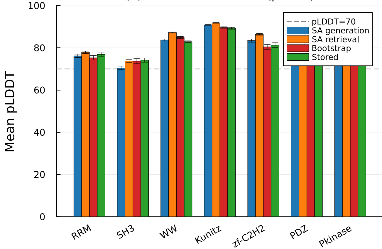
(A) ESMFold Confidence (pLDDT)
