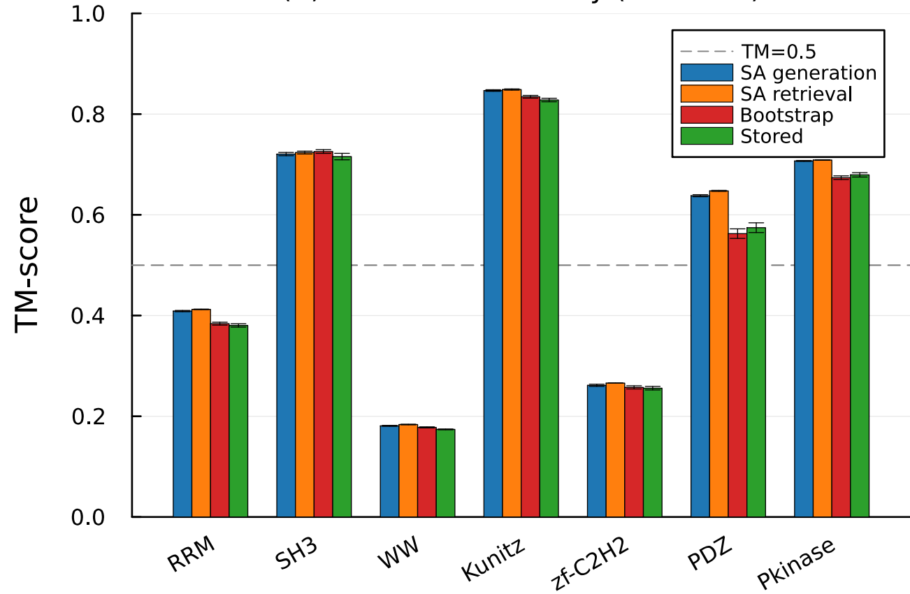
(B) Structural Similarity (TM-score)
