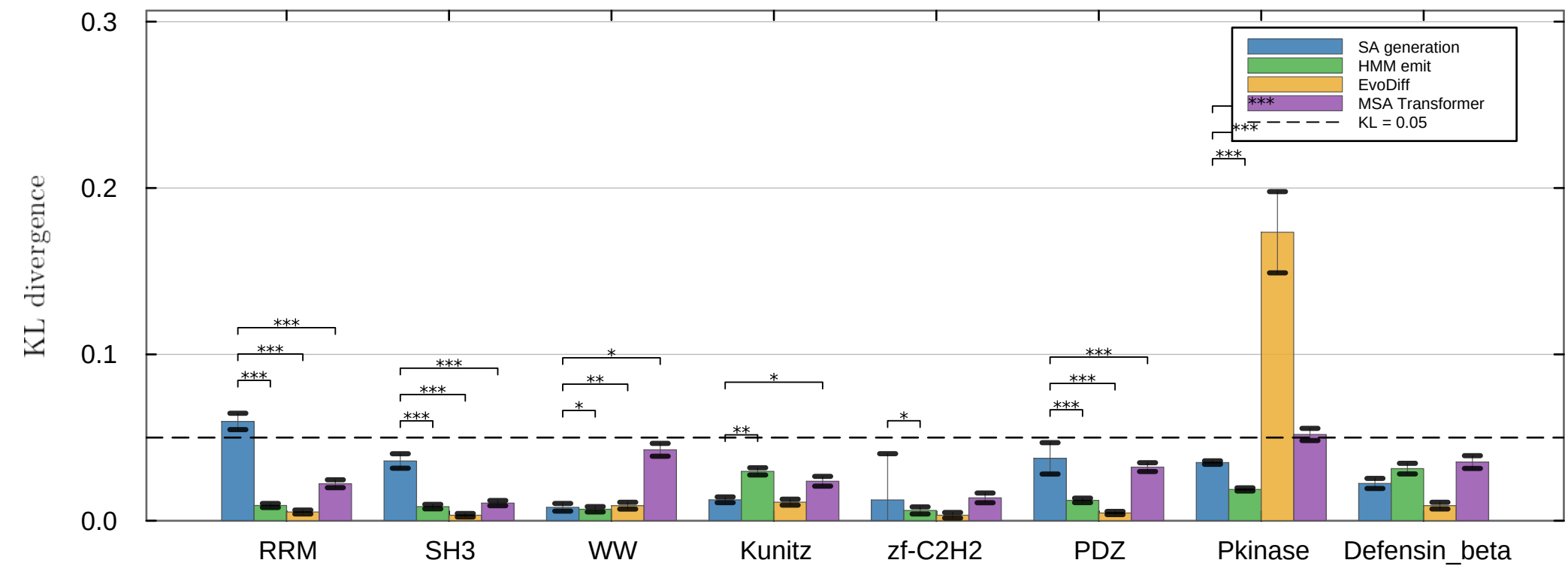
(A) AA composition fidelity (lower is better)
