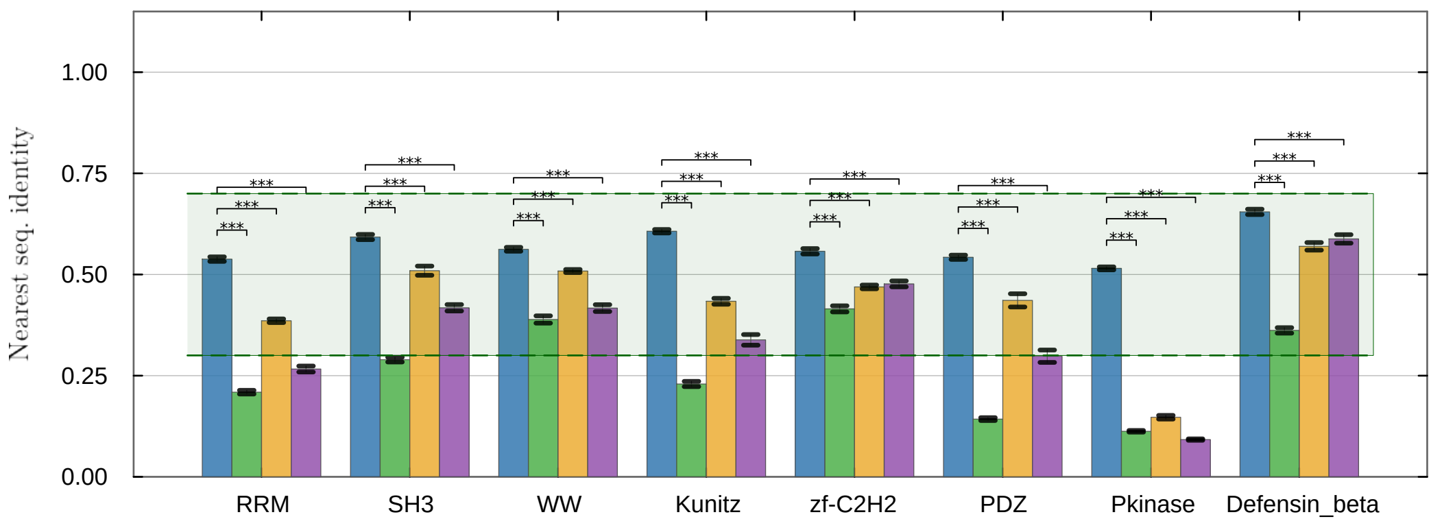
(C) Sequence identity (within-family target: 30-70%)
