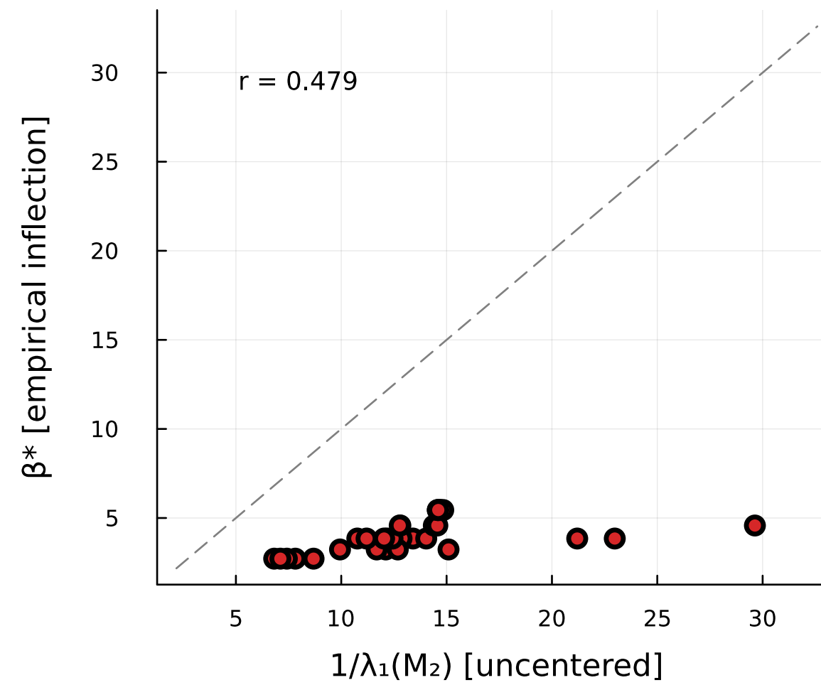
(B) Second Moment vs Empirical \beta^*
