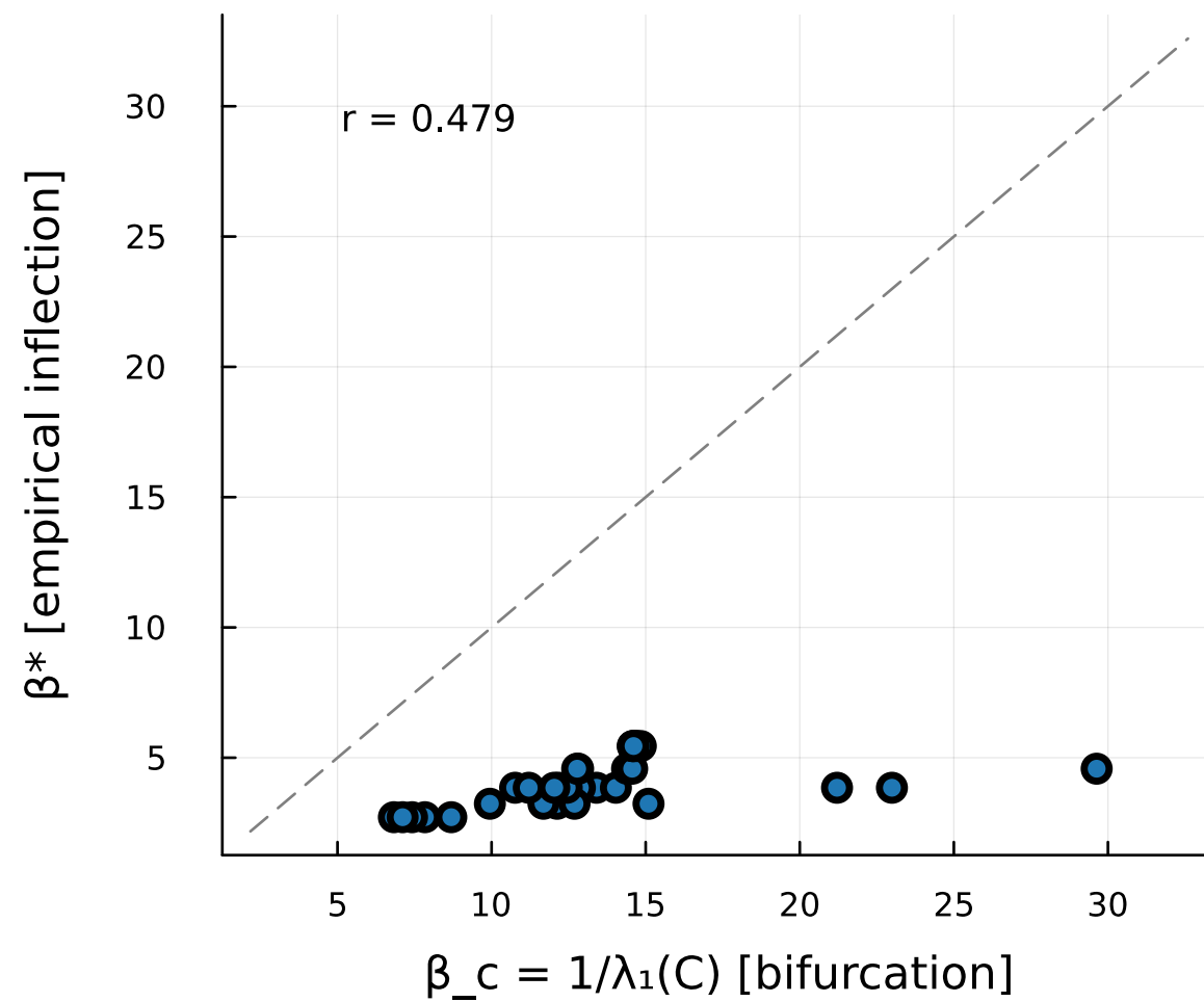
(A) Bifurcation vs Empirical \beta^*
