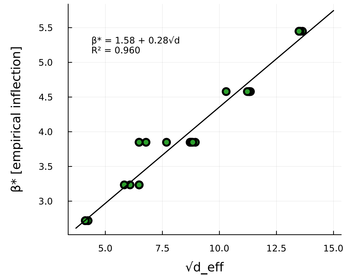
(C) \beta^* vs \sqrt{d\_eff}
