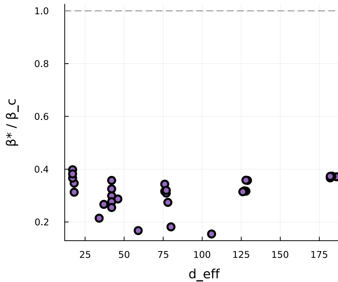
(E) Ratio \beta^*/\beta_c vs d\_eff
