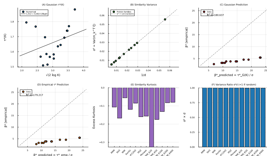
Figure S9: Analytical investigation of \beta^* . (A) Dimensionless softmax inflection \tau^*(K) for Gaussian scores. (B) Similarity variance \sigma^2 vs. 1/d for random probes; all points lie on the identity line. (C) Gaussian prediction \beta^*_{\text{pred}} = \tau^*_G(K)/\sigma vs. empirical \beta^* ; correct trend ( r = 0.98 ) but overshoots by \sim 4\times . (D) Same as (C) using the empirical \tau^* ; overshoot persists. (E) Excess kurtosis of the similarity distribution. (F) The ratio \sigma^2 d = 1 across all datasets, confirming \sigma^2 d = 1 .
