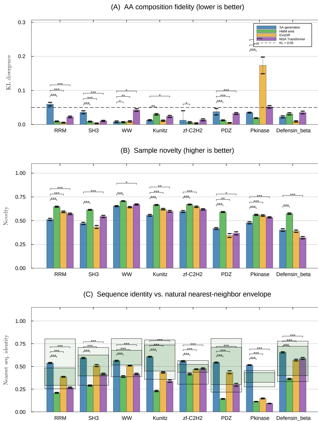
Fig. 3. Head-to-head comparison of SA generation against three learned baselines across all eight Pfam families. (A) KL divergence of amino acid composition (bootstrap SE; n_{\text{boot}}=1000 ); dashed line at \text{KL}=0.05 . (B) Novelty in PCA space. (C) Nearest sequence identity to a stored pattern; the green boxes show each family's natural within-family nearest-neighbor identity envelope (dark: 10th–90th percentile; light: full min–max range; SI Appendix, Table S14). Panels (B) and (C): per-chain means \pm 1 SE. Significance brackets: Wilcoxon rank-sum tests ( ***p < 0.001 , **p < 0.01 , *p < 0.05 ). Per-family numerical values are reported in SI Appendix for the learned baselines (Table S2) and for SA generation and the reference conditions (Table S1).
