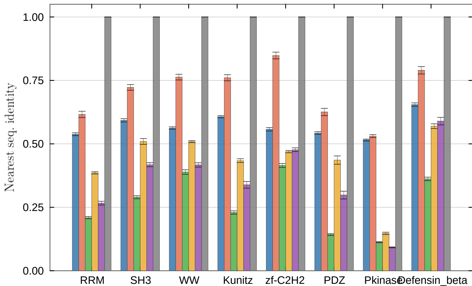
(C) Sequence identity
