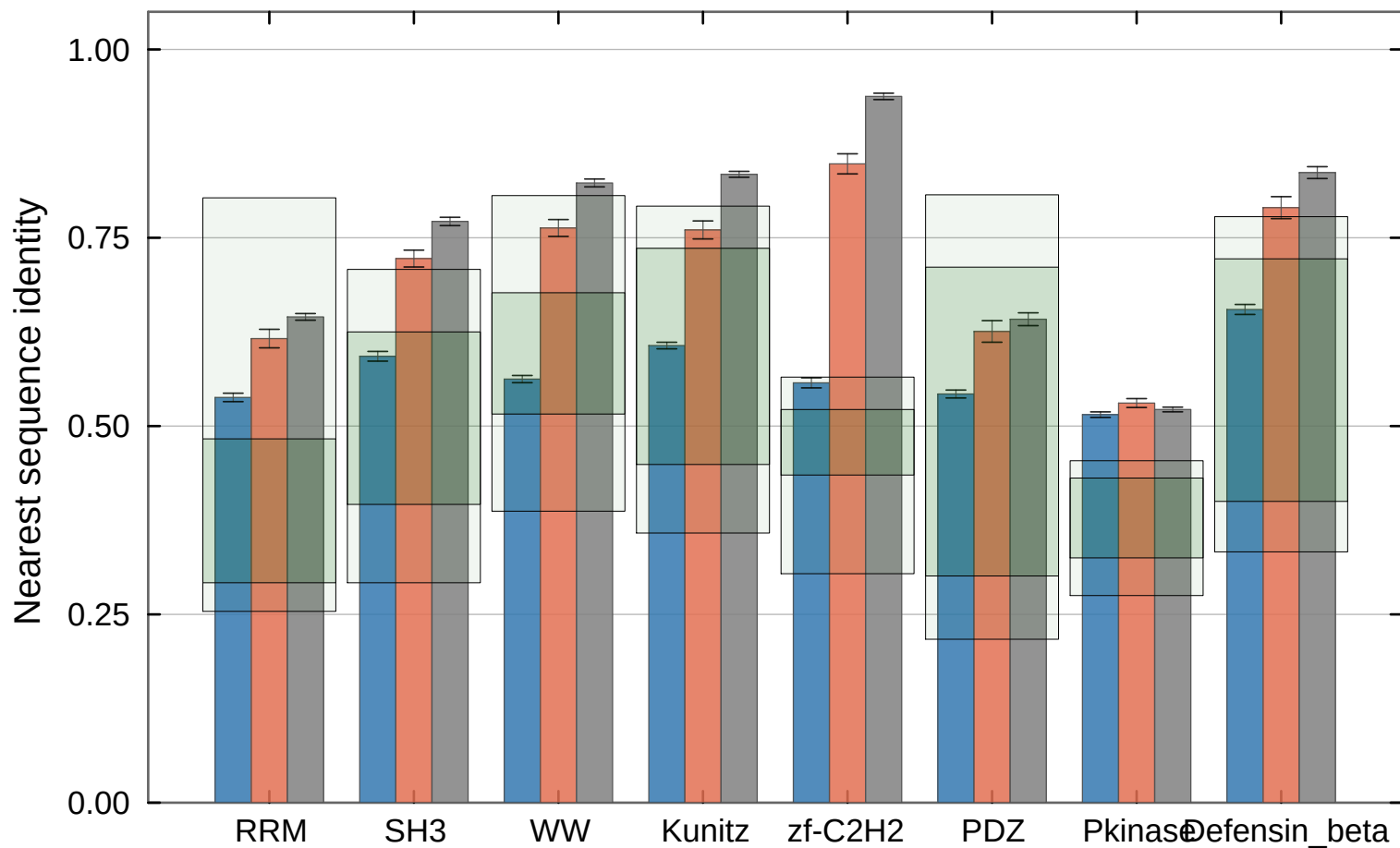
(C) Sequence identity vs. natural nearest-neighbor envelope
