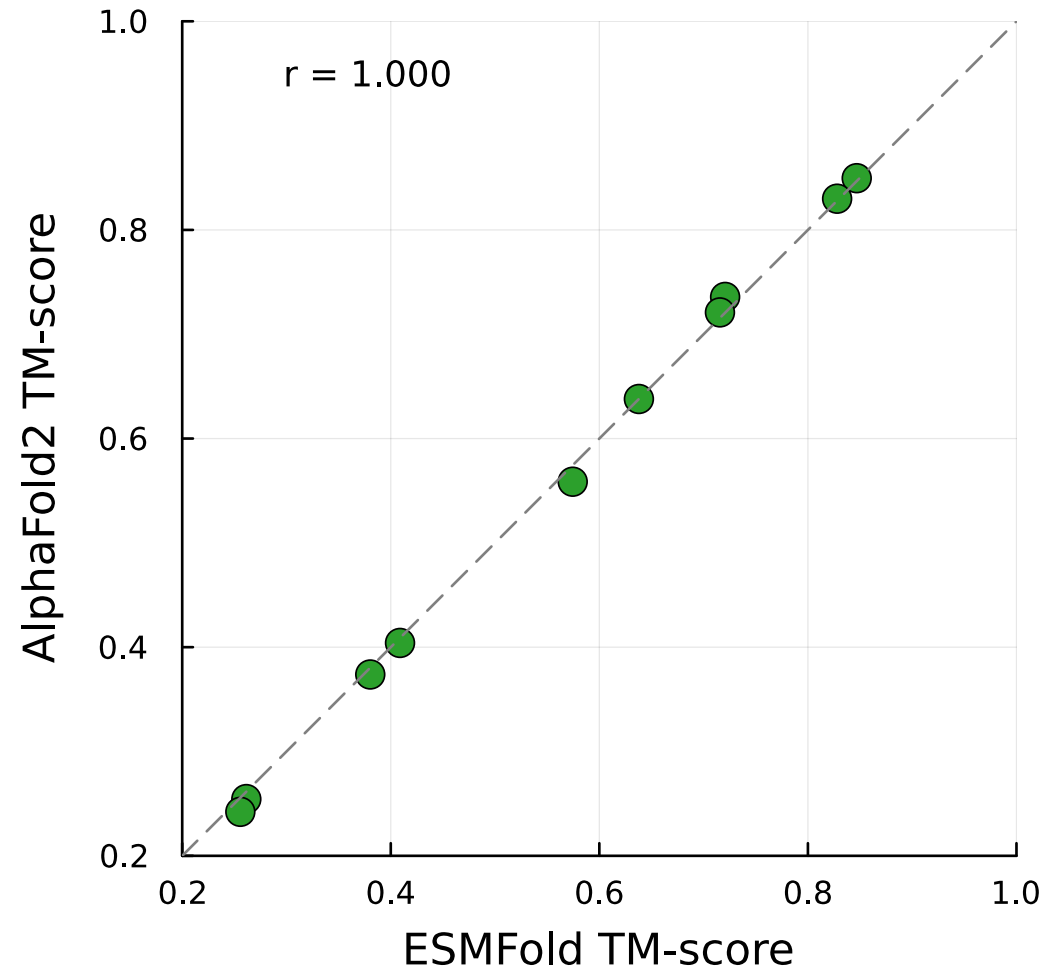
(B) TM-score Concordance
