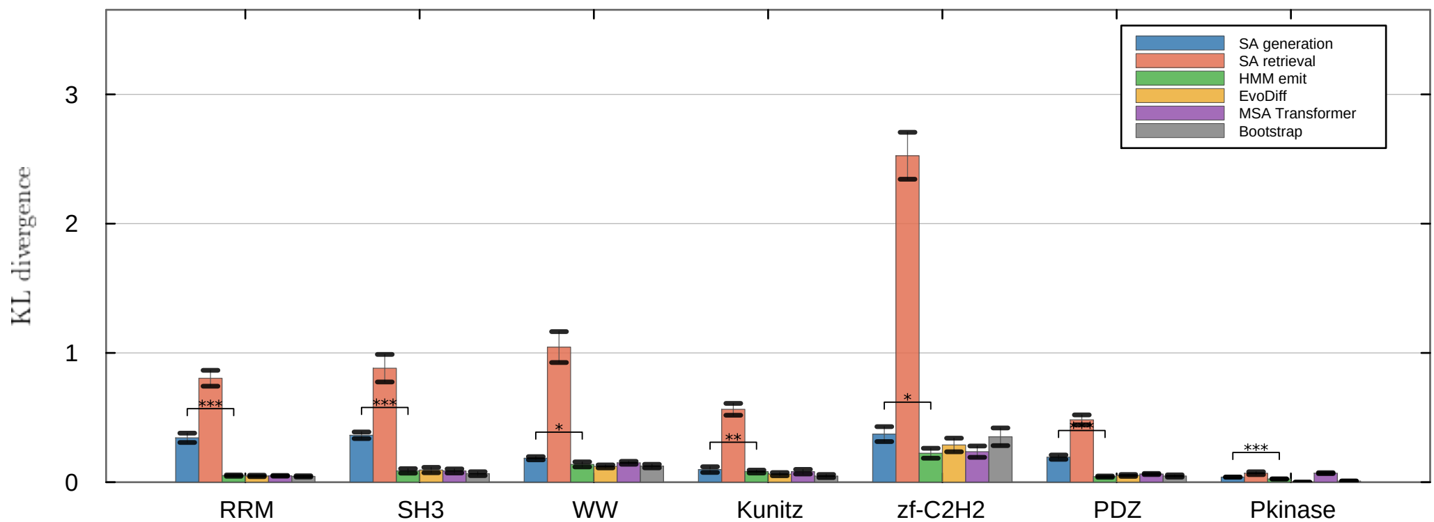
(A) AA composition fidelity
