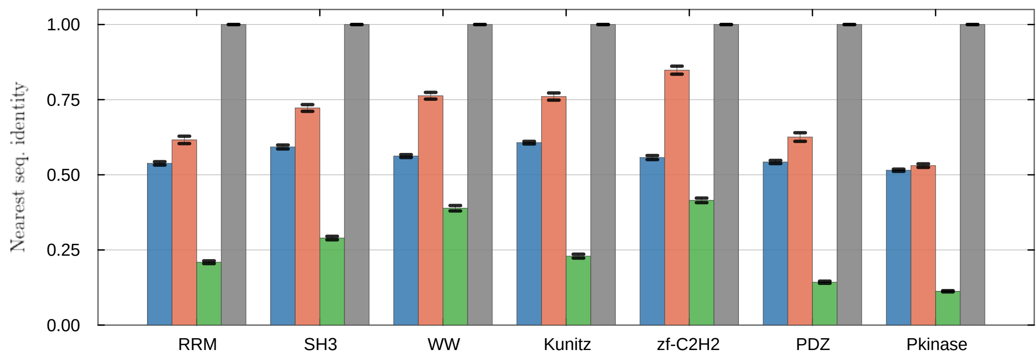
(C) Sequence identity
