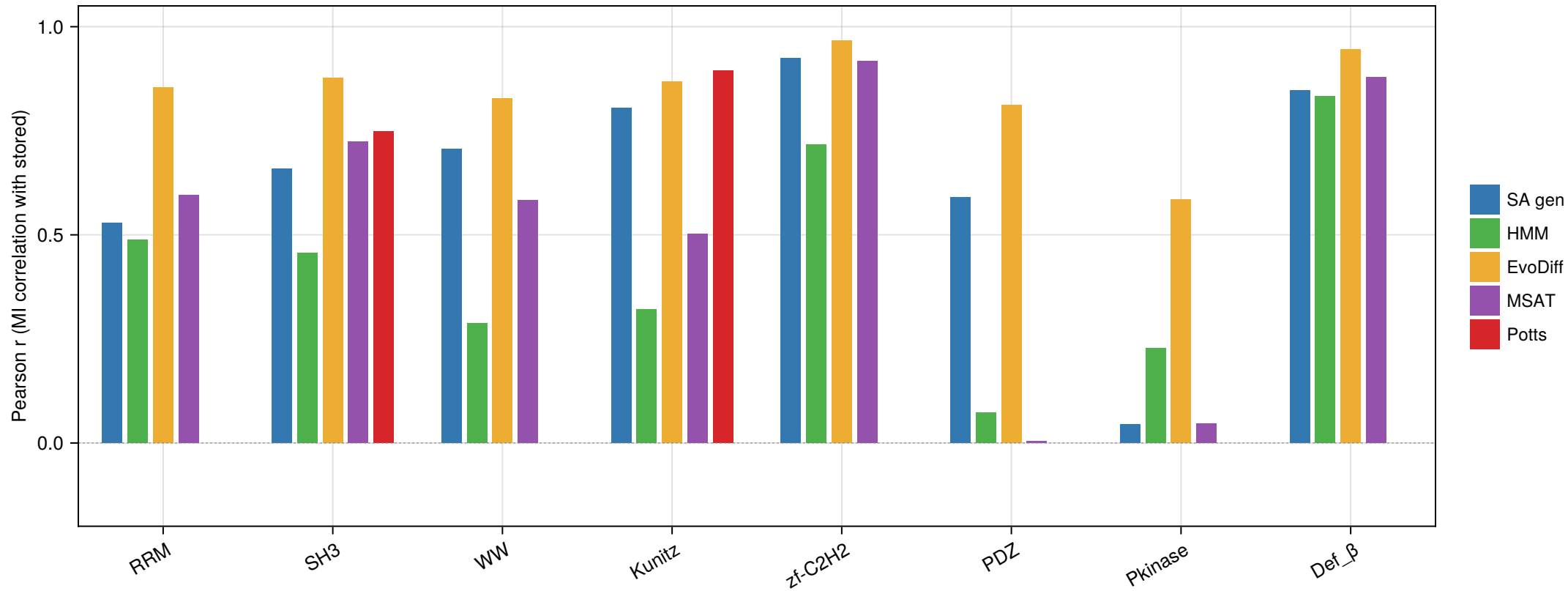
Pairwise MI preservation across families and methods
