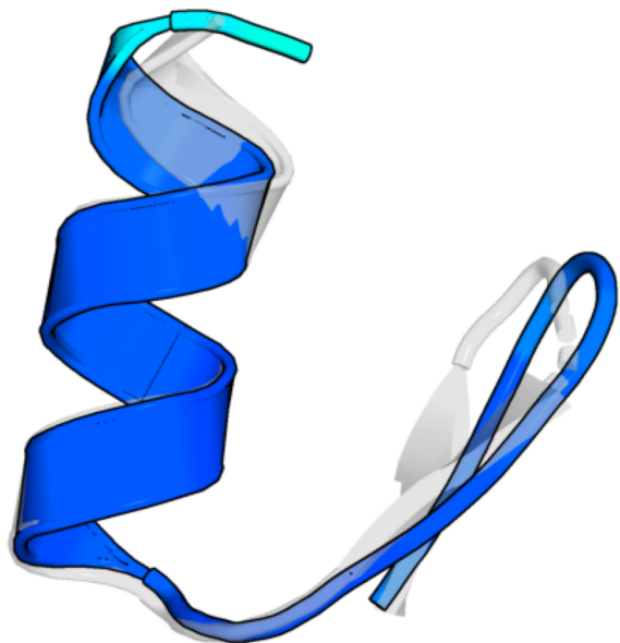
zf-C2H2
