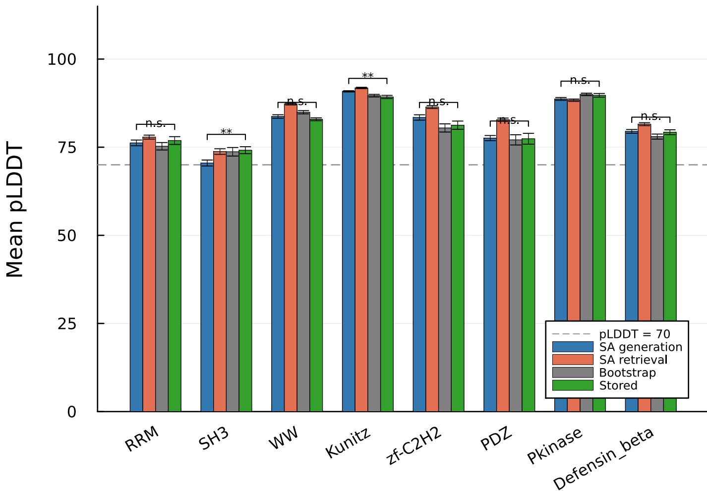
(A) ESMFold Confidence (pLDDT)
