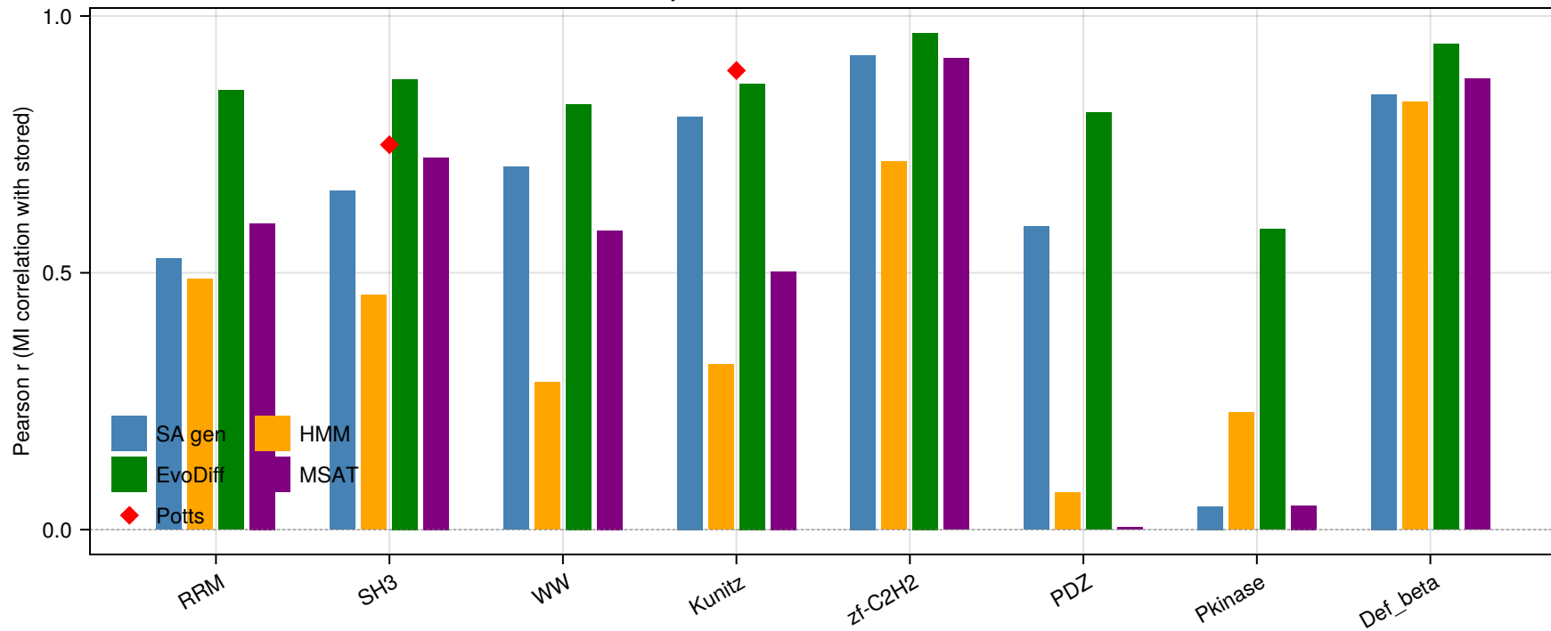
Pairwise MI preservation across families and methods
