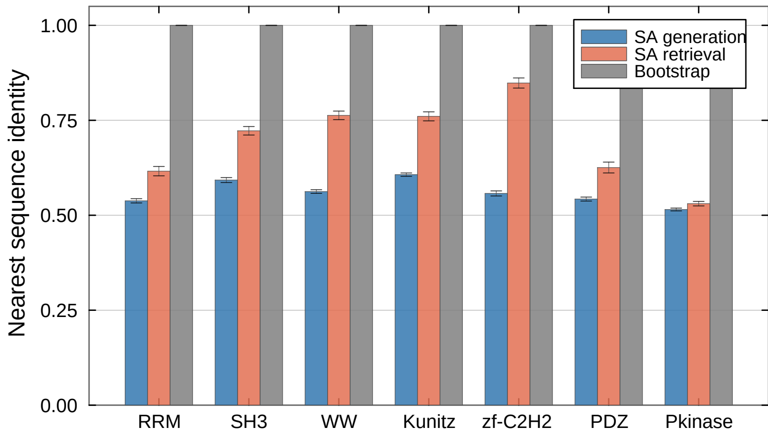
Sequence identity to nearest stored pattern
