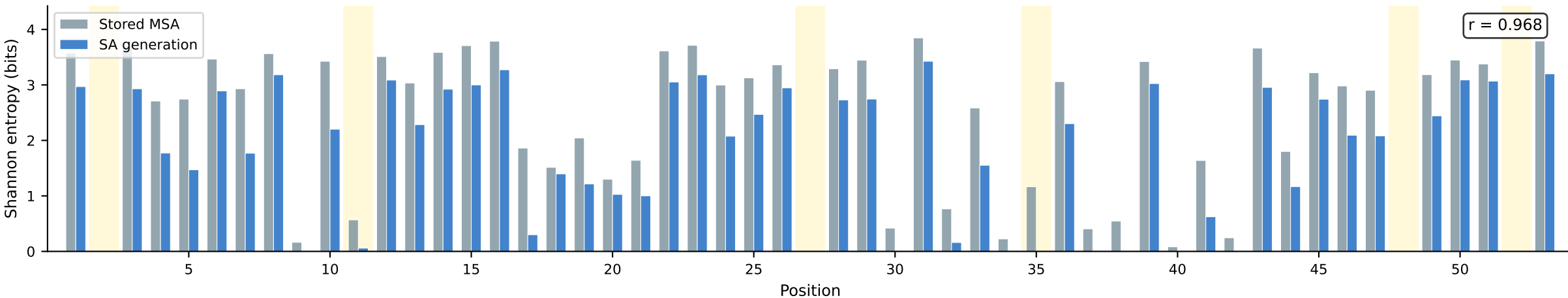
(B) Per-position entropy: stored MSA vs. SA-generated sequences
