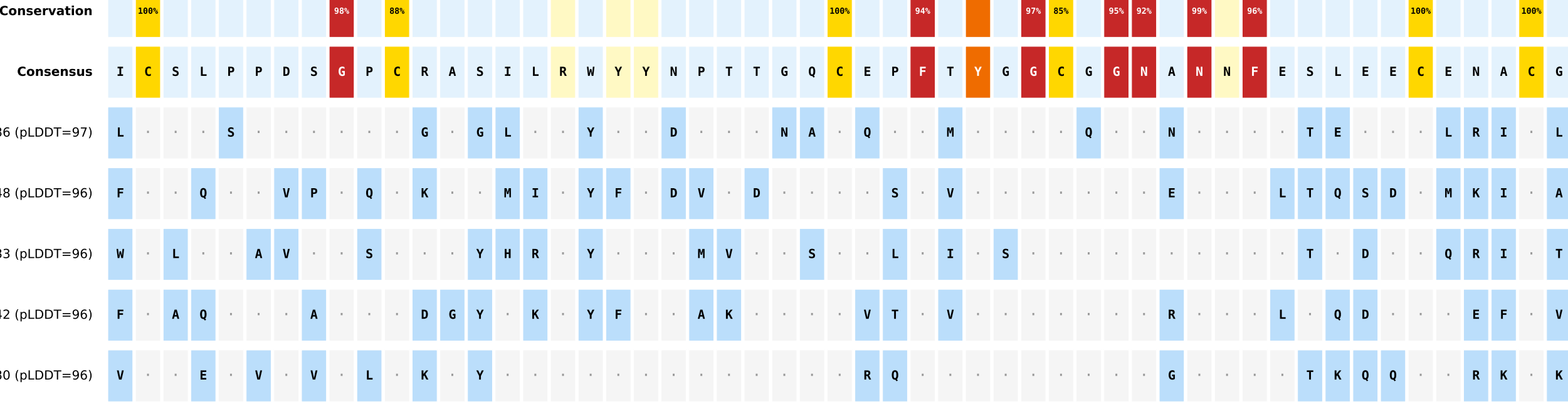
(A) Kunitz domain: consensus vs. top SA-generated sequences
