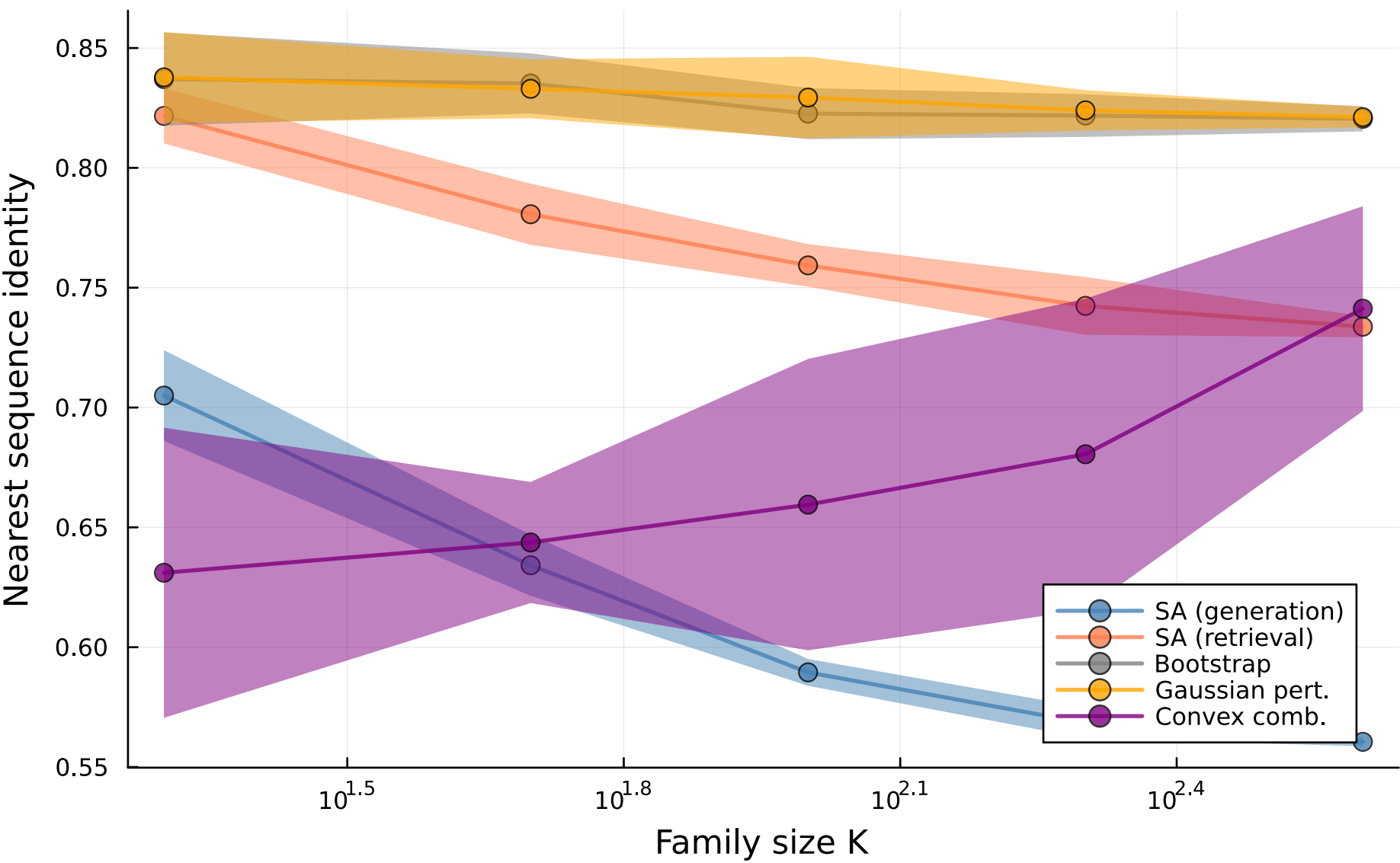
Sequence Identity vs. Family Size
