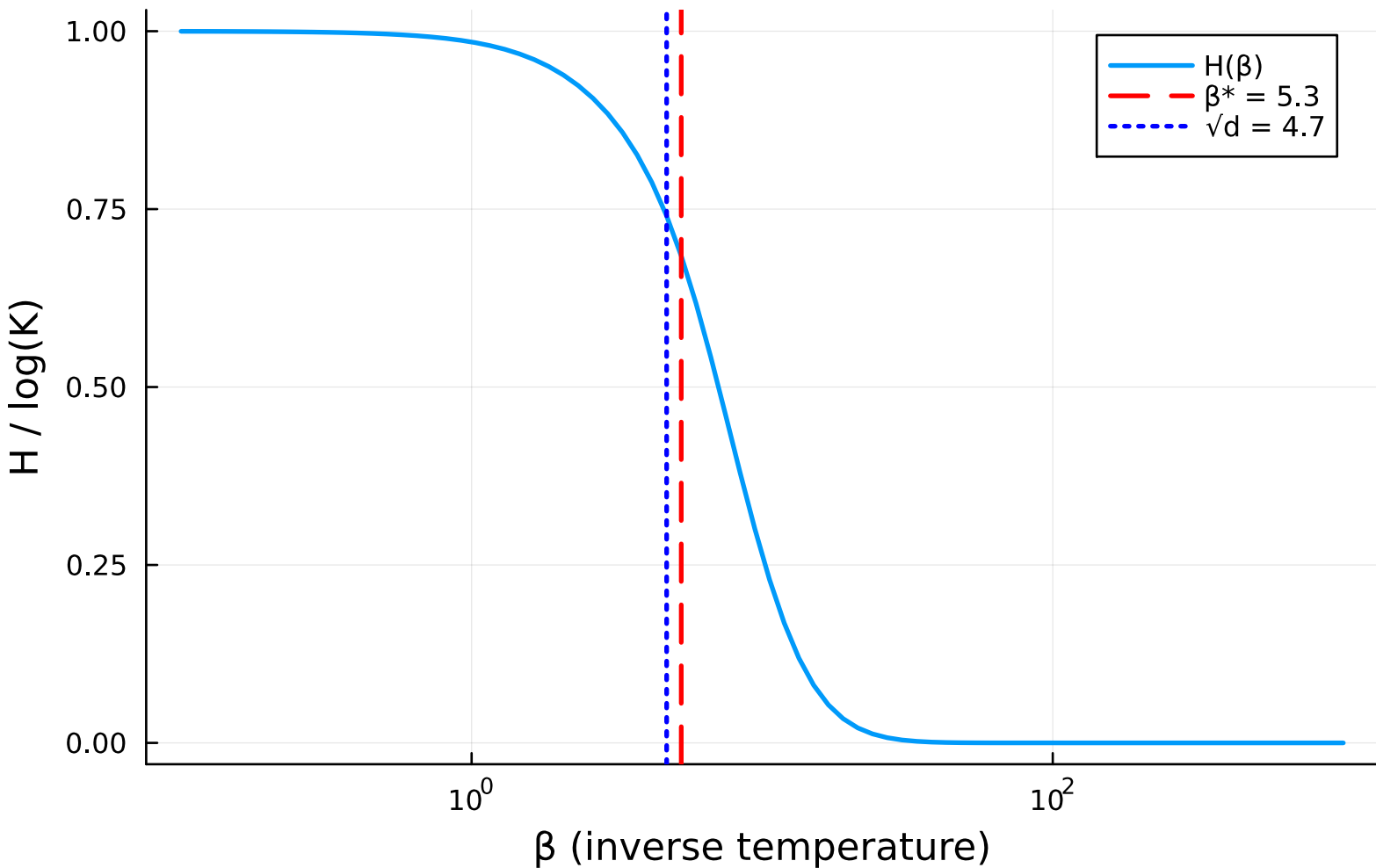
Attention Entropy vs \beta ( d=22 , K=116 )
