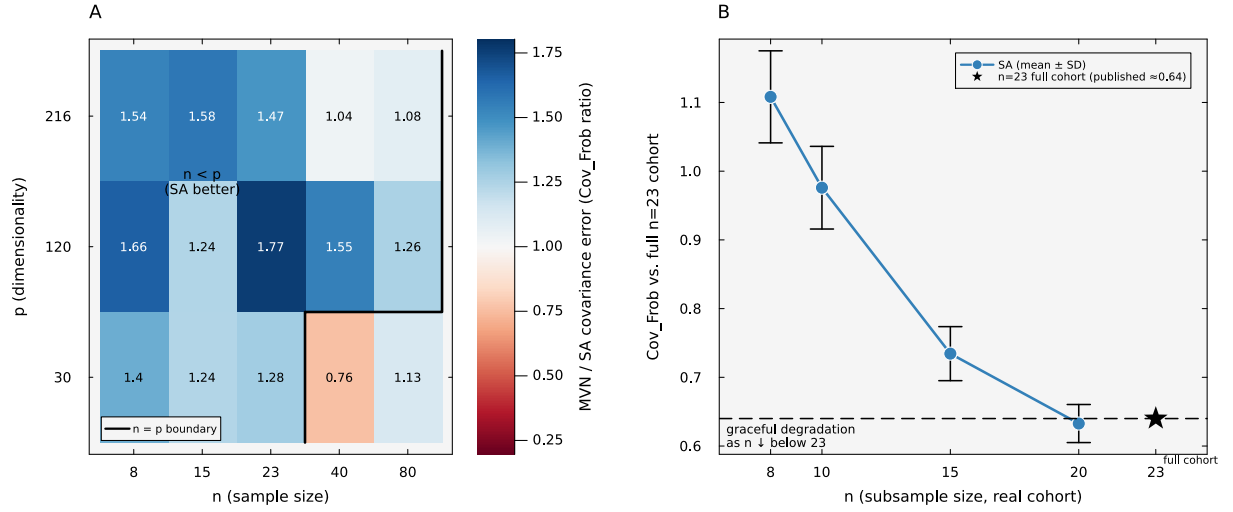
Figure 4: Population recovery and clinical-cohort subsampling. (A) For each low-rank Gaussian setting, stochastic attention and a sample-covariance Gaussian generator were fit to the same simulated training cohort and each generated 100 profiles. Color represented the ratio of their relative Frobenius errors against the known population covariance (Gaussian error divided by stochastic-attention error), averaged over latent ranks 3, 5, and 10. Values above one (blue) indicated lower error for stochastic attention. Because the target covariance was fixed before the training cohort was drawn, this measured population recovery rather than reproduction of the training data. (B) Stochastic attention was fit to ten random subsets of the clinical cohort at each of n=20, 15, 10 , and 8 , and each fit generated 100 profiles. Points and bars represented the mean and standard deviation of the relative cross-visit correlation error against the same full 23-patient reference; the star represented the fit using all 23 patients.
