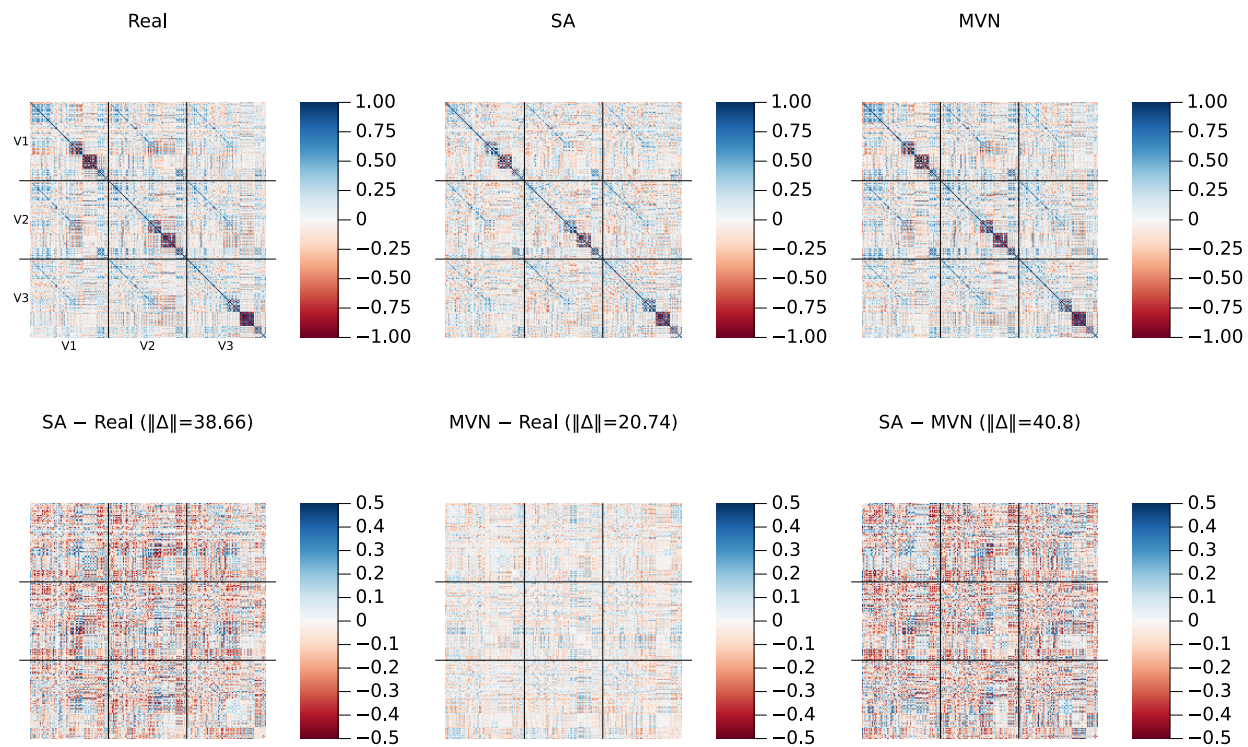
Supplementary Figure 1: Cross-visit correlation structure (amplified residual scale) . Same layout as the main-text correlation figure, but with the bottom-row residual panels plotted on a \pm 0.5 color scale (vs. \pm 1.0 in the main text) to reveal fine structure. Frobenius norms of each residual matrix are shown in the panel titles.
