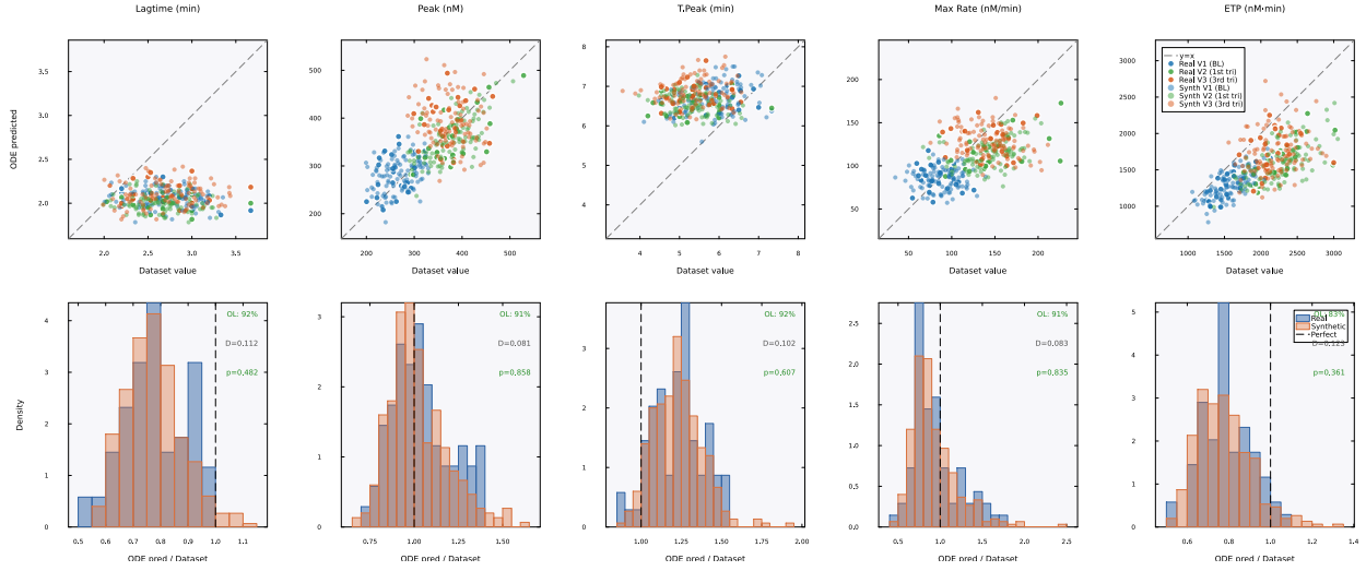
Figure 6: Mechanistic validation (TF-only). Top row: BZ2012 ODE-predicted TGA values (vertical axis) versus dataset TGA values (horizontal axis) for five thrombin generation parameters. The dataset values are the TGA measurements from each patient’s record, present for both real and synthetic patients. The ODE-predicted values are computed by running each patient’s coagulation factor levels through the 58-species BZ2012 model. The dashed line indicates where the ODE model would perfectly reproduce the dataset value ( y=x ); systematic deviations from this line (e.g., lagtime underprediction) reflect ODE model bias, not synthetic data failure. Filled markers are real patients, open markers are SA-generated synthetic patients, colored by visit: blue (V1/baseline, training set), green (V2/first trimester), orange (V3/third trimester). Real and synthetic patients occupy the same cloud with the same pattern of ODE model bias. Bottom row: ODE-predicted/dataset ratio distributions for real (blue) and synthetic (orange) patients. If SA had generated biologically implausible factor combinations, the ODE model would process them differently, producing divergent ratio distributions. Instead, the distributions overlap substantially. Each panel is annotated with cloud overlap (OL), the two-sample Kolmogorov–Smirnov statistic ( D ), and p -value. All five features show p > 0.35 , confirming that the ODE model cannot distinguish real from synthetic patients.
