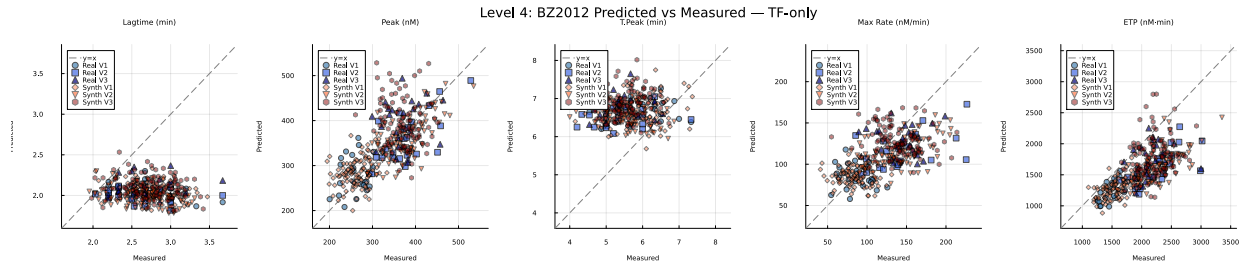
Figure 6: Mechanistic model predicted versus measured TGA features (TF-only). Each panel shows one TGA feature; the dashed line indicates perfect prediction ( y=x ). Blue markers: real patients (circles = V1/train, squares = V2, triangles = V3). Red/brown markers: SA-generated synthetic patients (diamonds = V1, inverted triangles = V2, hexagons = V3). Synthetic patients occupy the same predicted-versus-measured cloud as real patients across all features and visits.
