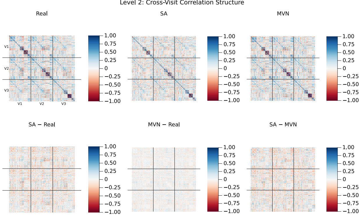
Figure 3: Cross-visit correlation structure. Top row: full 216 \times 216 Pearson correlation matrices for Real ( K=23 , left), SA ( N=100 , center), and MVN ( N=100 , right) populations. Each matrix is organized as a 3 \times 3 grid of 72 \times 72 blocks (delineated by black lines), where the diagonal blocks capture within-visit feature correlations (V1-V1, V2-V2, V3-V3) and the off-diagonal blocks capture cross-visit dependencies (e.g., V1-V3: does a patient’s baseline Factor VIII predict their third-trimester Factor VIII?). SA preserves both the within-visit and cross-visit block structure. Bottom row: pairwise residual matrices (element-wise subtraction), all plotted on the same \pm 1 color scale as the top row. The SA-Real residual shows small, unstructured deviations distributed throughout. The MVN-Real residual is notably smoother—particularly in the off-diagonal blocks—reflecting the Ledoit-Wolf regularization that systematically shrinks cross-visit correlations toward zero. The SA-MVN residual confirms that the two methods differ most in precisely these off-diagonal blocks, where SA retains longitudinal dependencies that MVN’s rank-deficient covariance estimate cannot represent. A version with amplified residual color scale ( \pm 0.5 ) and Frobenius norms is provided in Supplementary Fig. S1.
