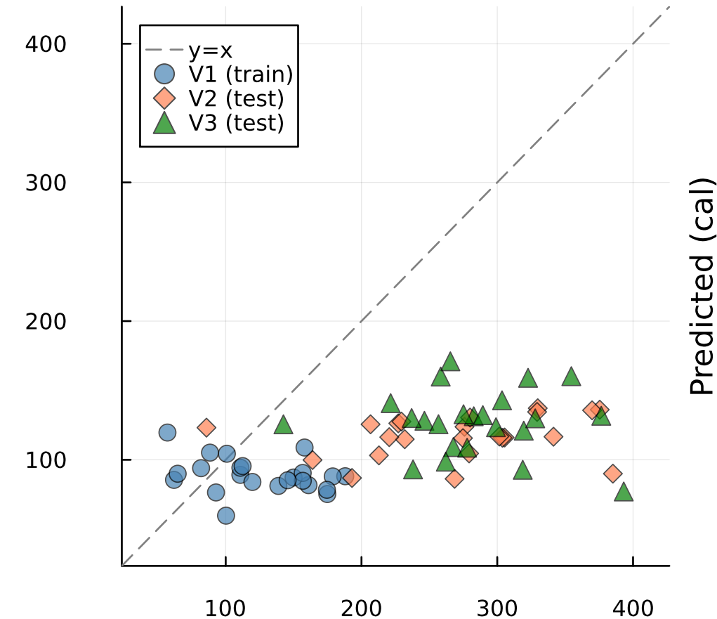
Peak (nM)
