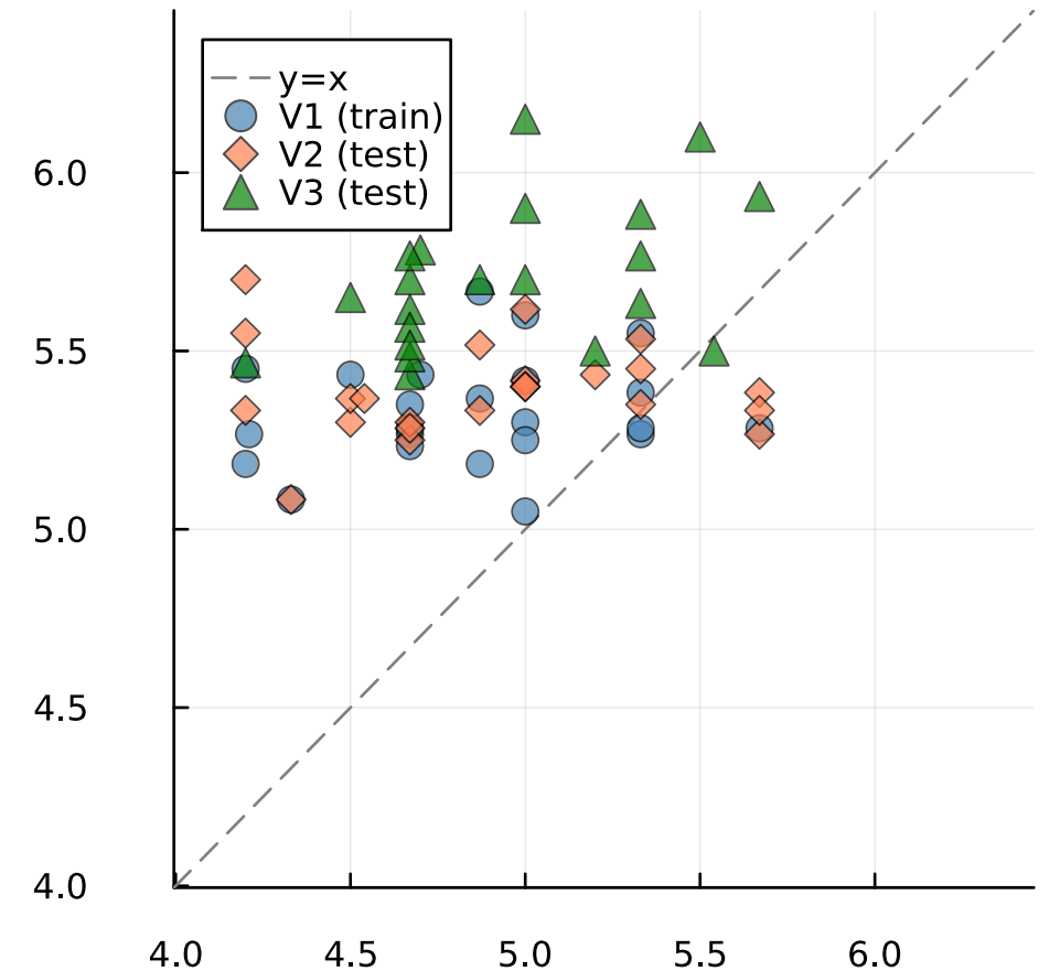
T.Peak (min)
