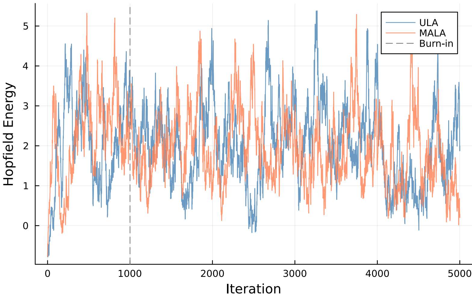
ULA vs MALA Energy Traces (Chain 1)
