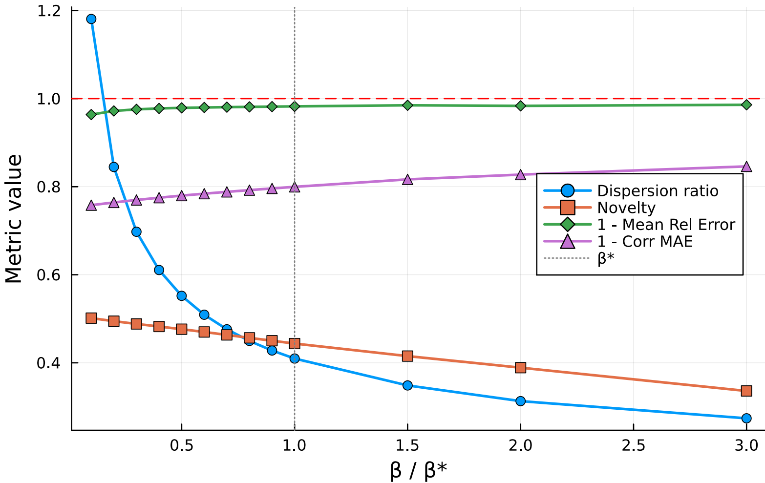
\beta Sweep: Dispersion-Fidelity Tradeoff
