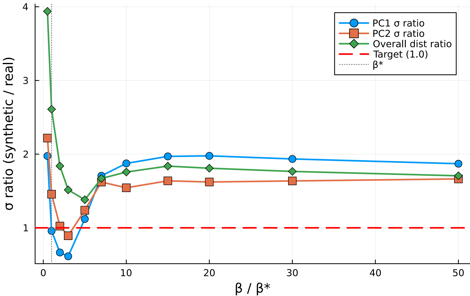
Raw PCA: Dispersion vs \beta
