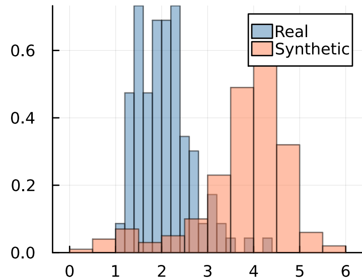
TNF \alpha R2
