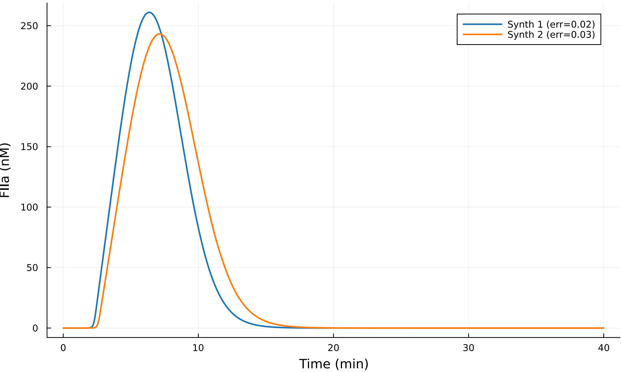
BST Model Fit — Synthetic Patients (Visit 1)
