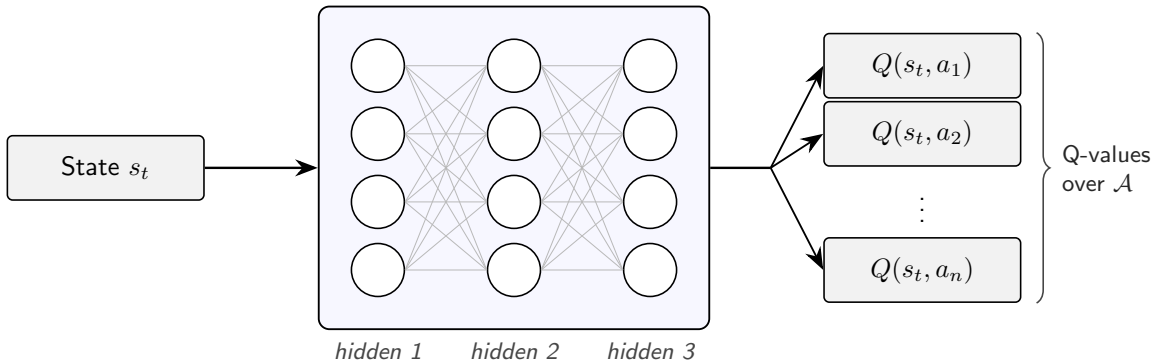
Q-network with parameters \theta
