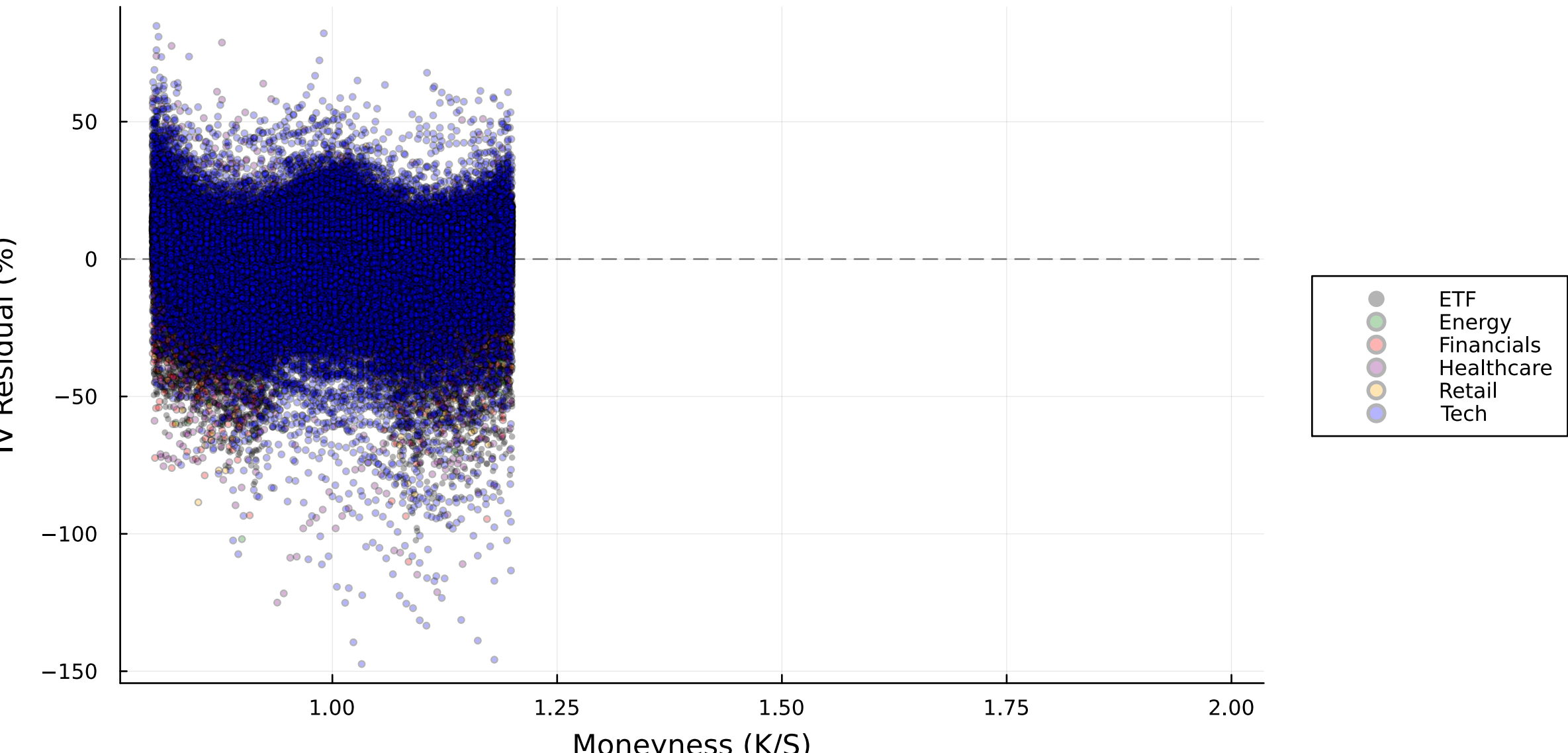
IV Residuals (Model - Market) by Moneyvness
