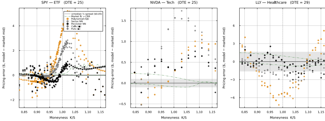
Figure 2: Model-vs-market dollar pricing error (CRR American at the calibrated IV minus market mid) versus moneyness for SPY, NVDA, and LLY at one representative DTE per ticker. Four model tiers are overlaid on each panel: parametric \psi (light), sector \psi_{NN} (medium), per-ticker \psi_{NN} (dark), and market-IV reference (gray, by construction near zero). The per-ticker fit collapsed the dollar error to within \$1 of the market mid across the tradeable moneyness range on all three names.
