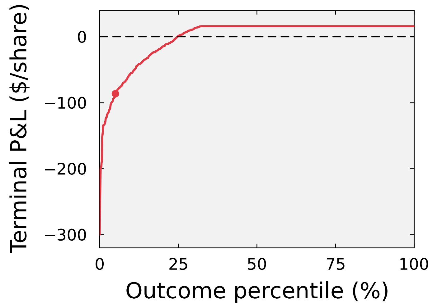
(b) GS Call
