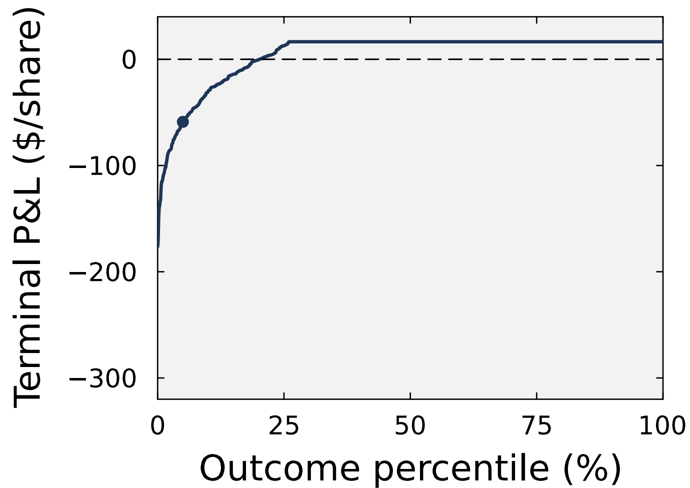
(a) GS Put
