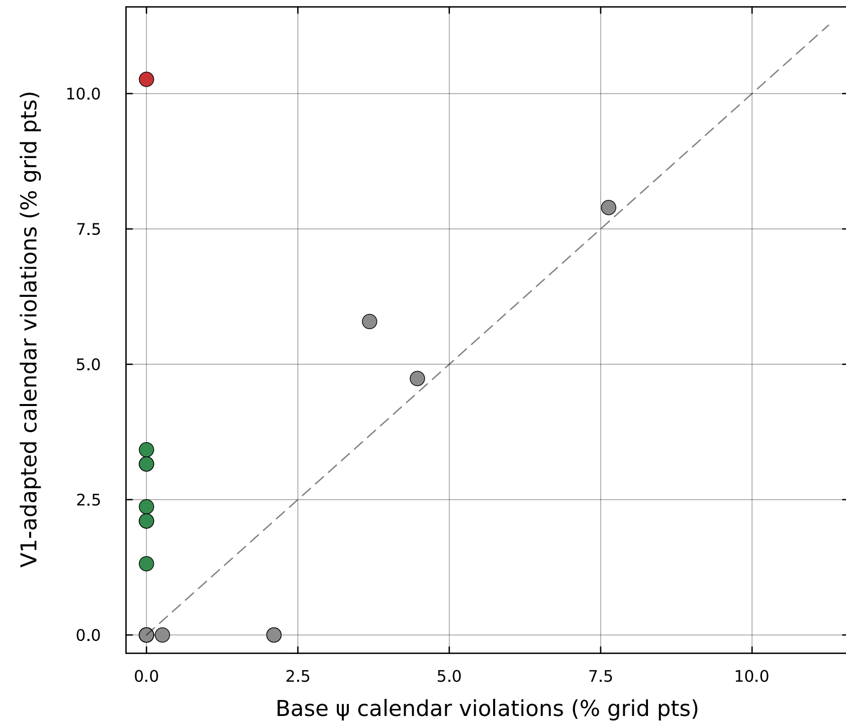
Calendar arbitrage: adapted vs base
