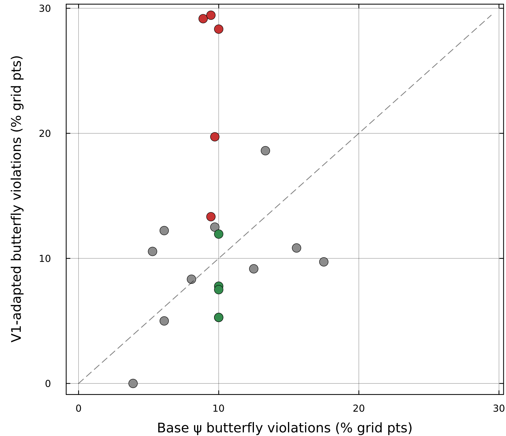
Butterfly arbitrage: adapted vs base
