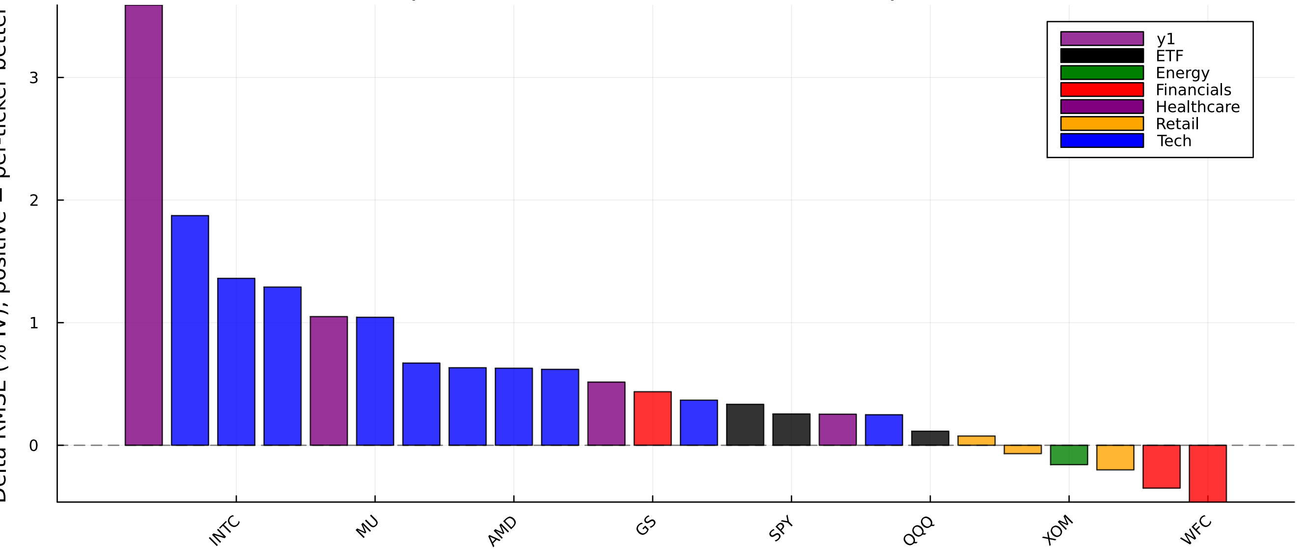
Per-Ticker NN Improvement Over Sector NN (in-sample RMSE reduction)
