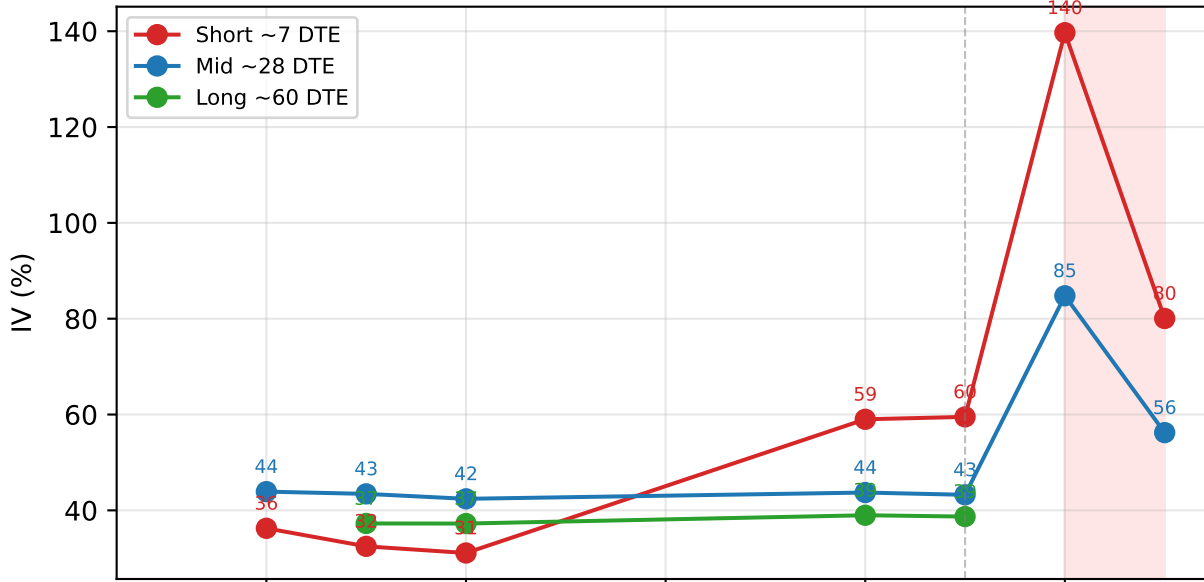
QCOM (ATM IV, moneyness \in [0.97, 1.03] )
