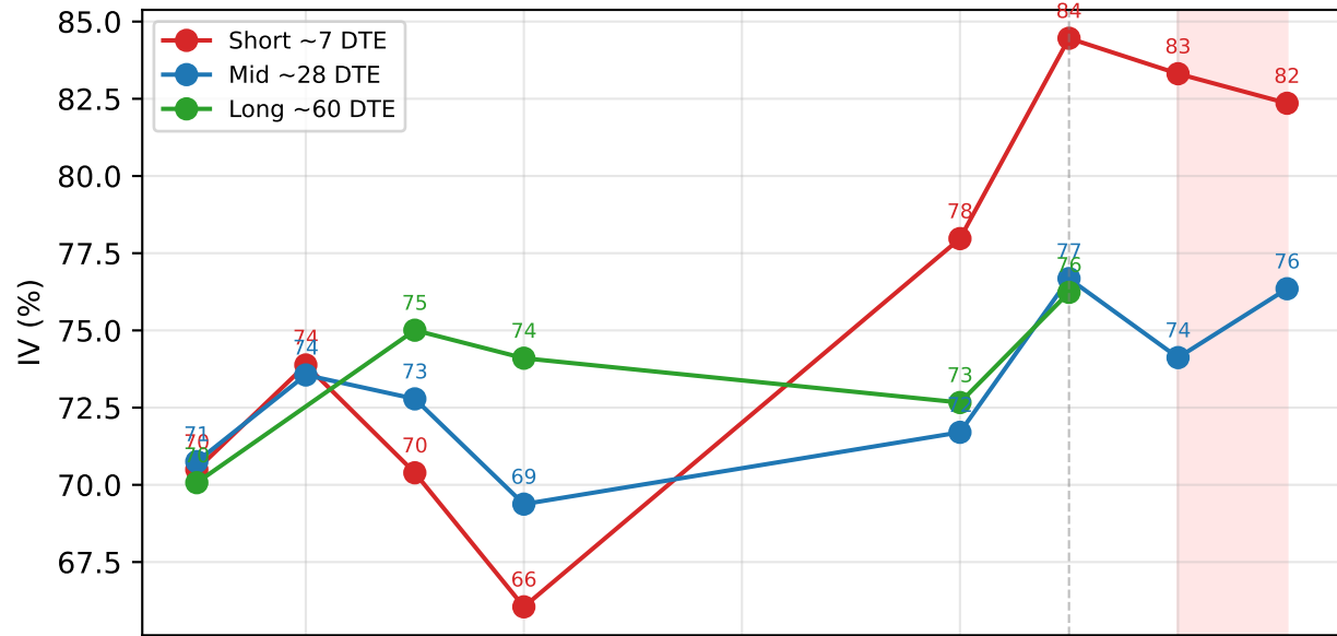
MU (ATM IV, moneyness \in [0.97, 1.03] )
