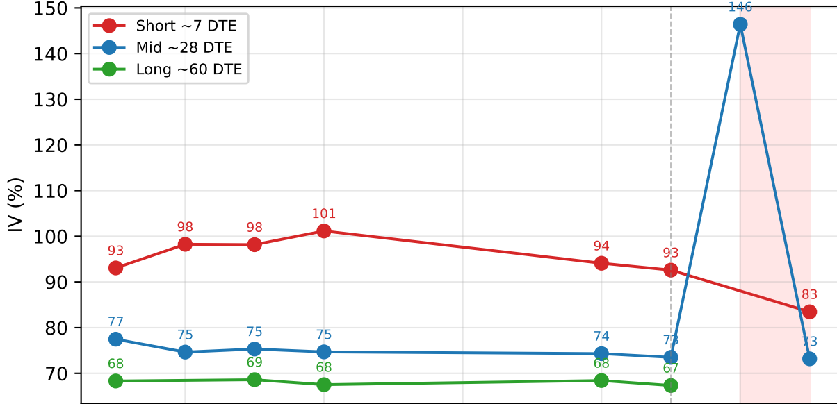
INTC (ATM IV, moneyness \in [0.97, 1.03] )
