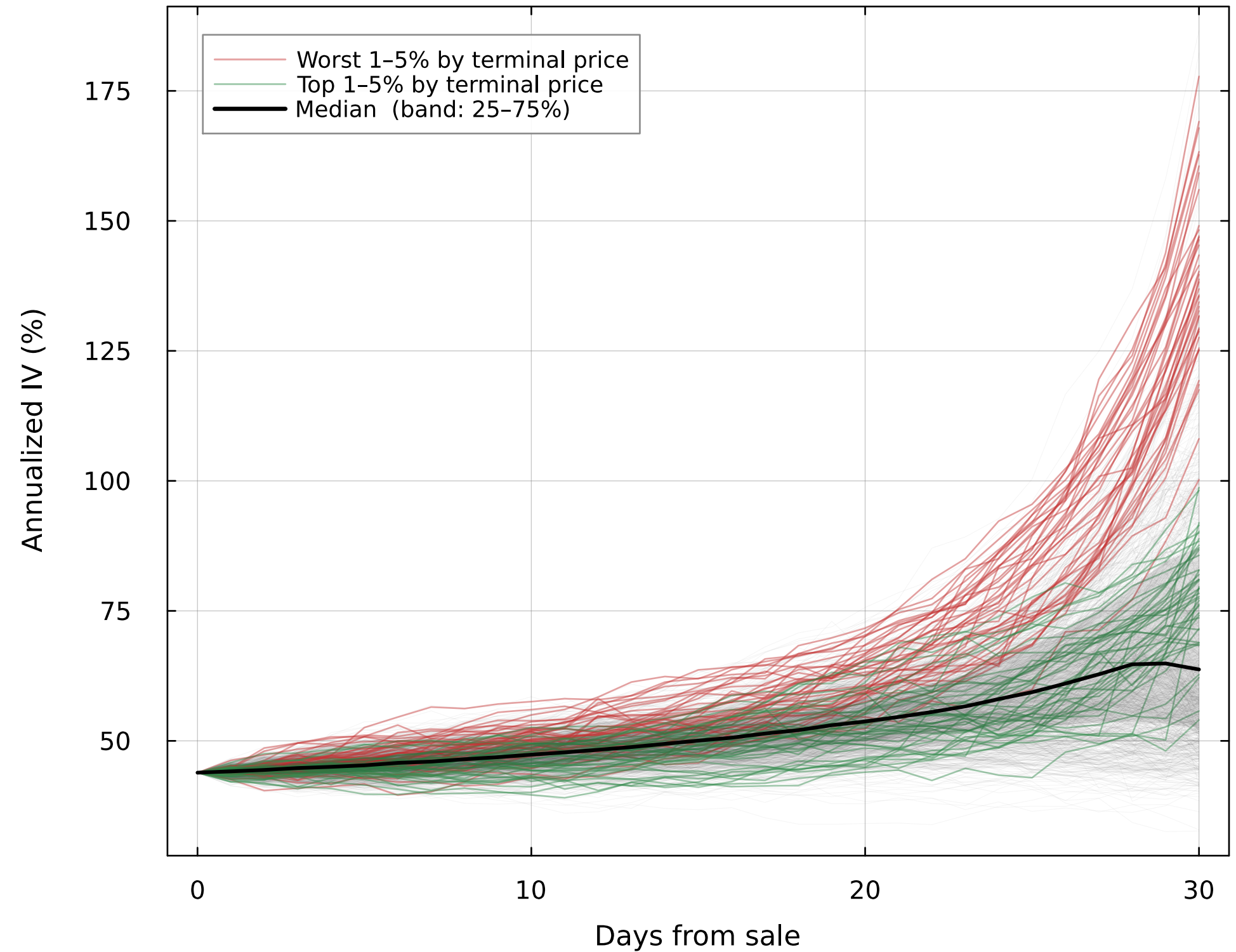
Implied volatility at the call strike (K = $940.0)
