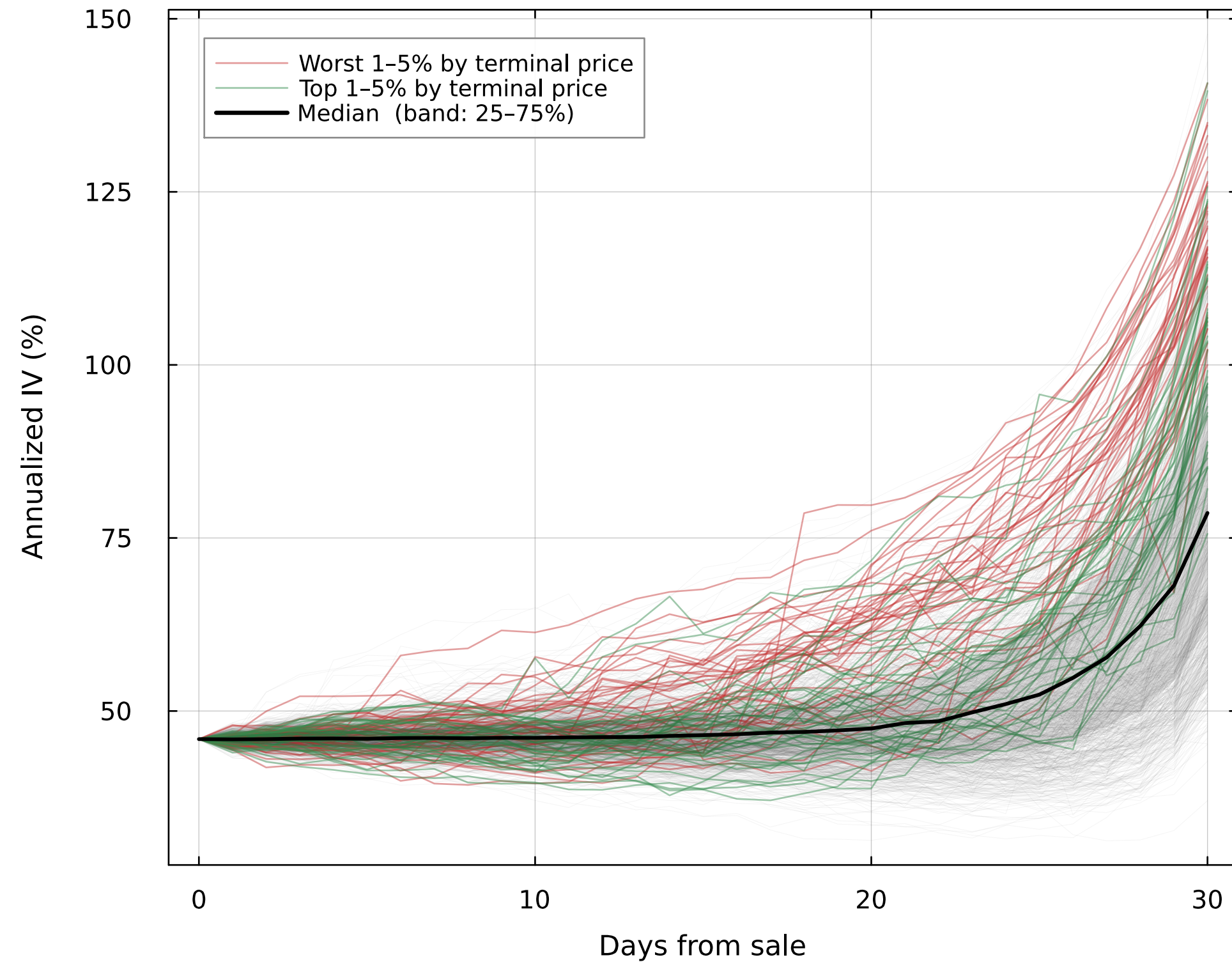
Implied volatility at the call strike (K = $435.0)
