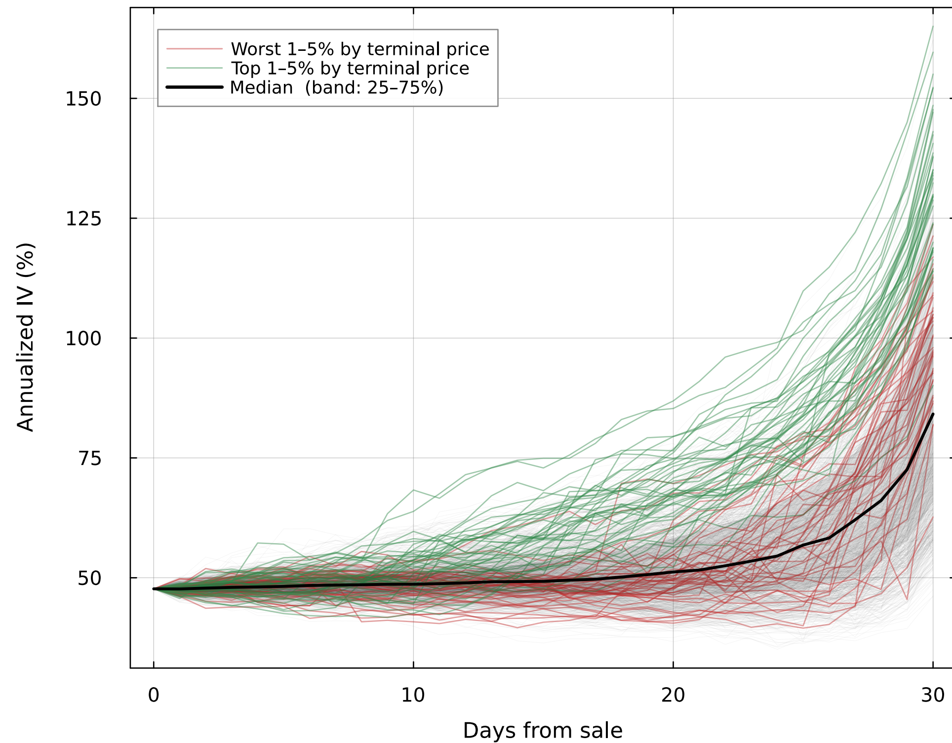
Implied volatility at the put strike (K = $375.0)
