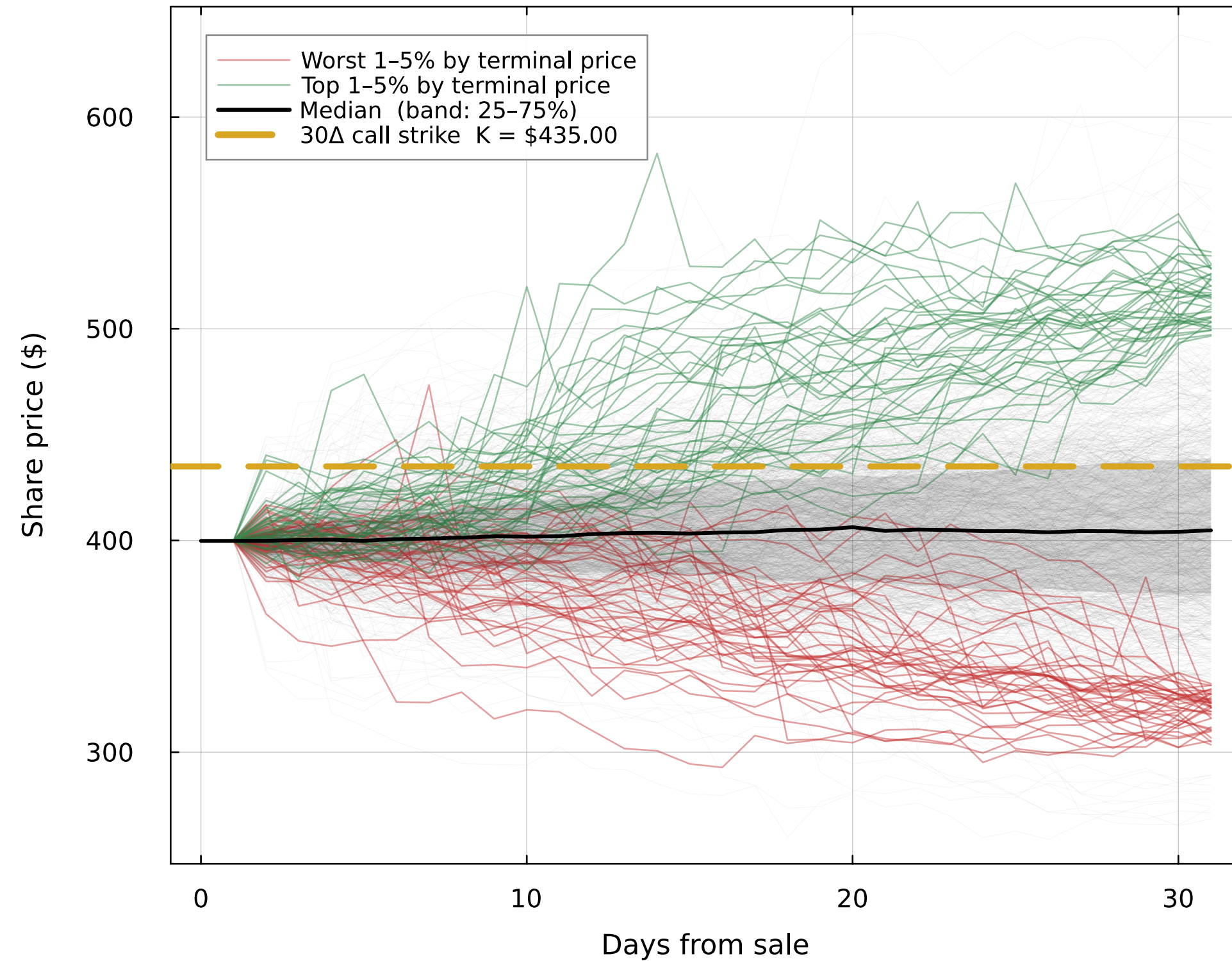
AVGO share price paths ( S_0 = \$399.83 )
