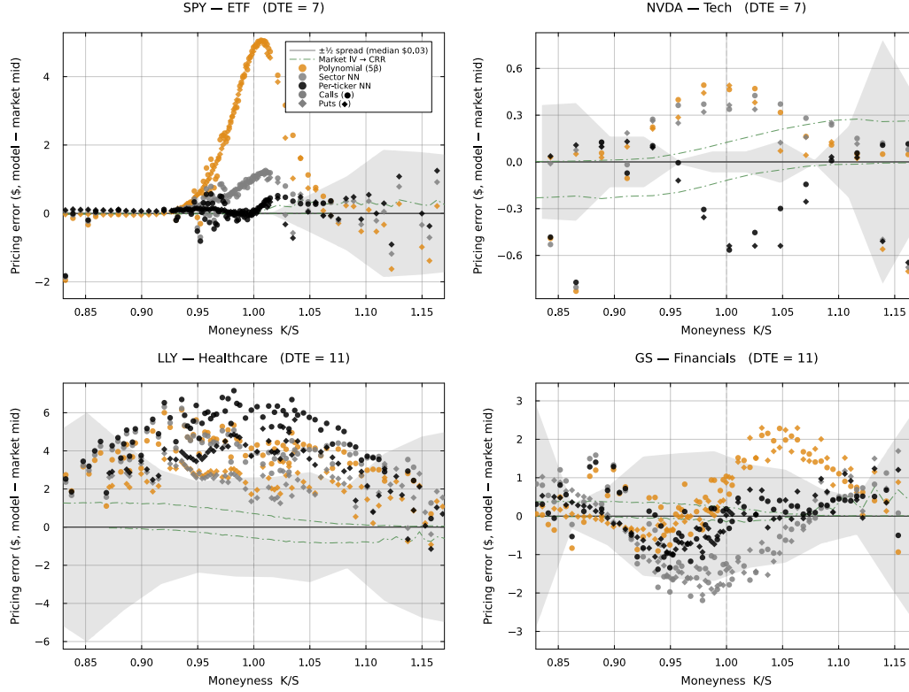
Figure 2: In-sample comparison of CRR American-option prices with market mids across moneyness for SPY, NVDA, LLY, and GS on May 11, 2026. Errors are lattice price minus market mid. Curves show the parametric, sector, per-ticker, and market-IV reference inputs. The gray ribbon is the median local bid-ask half-spread by moneyness bin. A point inside the ribbon has an absolute pricing error below that local half-spread.
