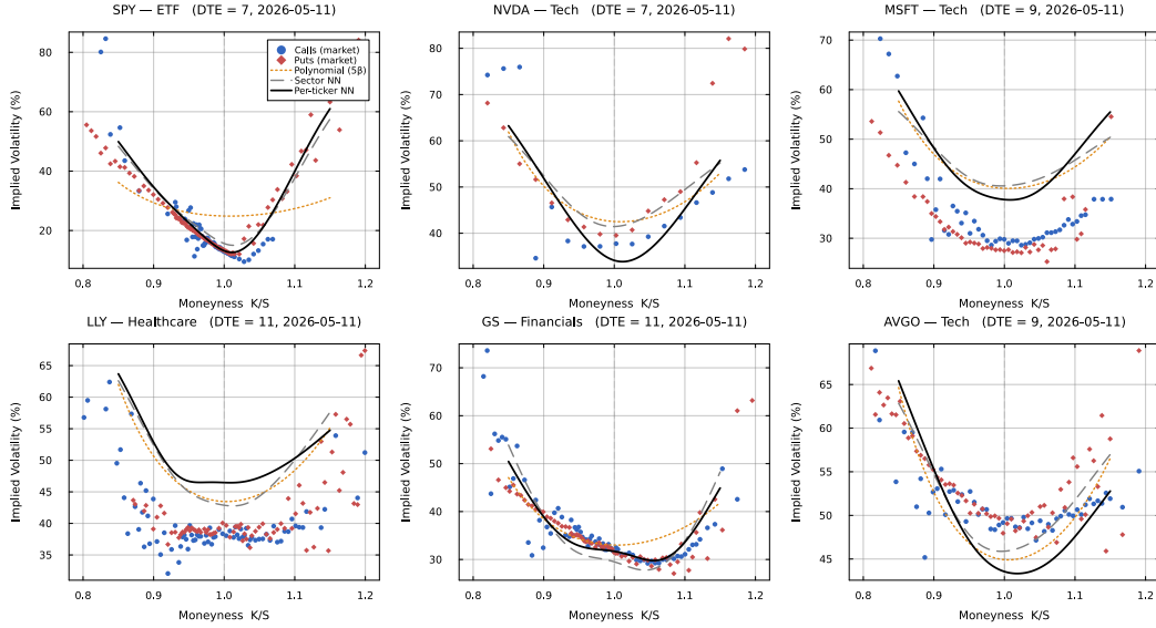
Figure 1: Fitted IV smiles for six representative tickers at a middle maturity. Points show market IV, the solid curve shows the per-ticker neural surface, and the dashed curve shows the sector surface. All observations came from the fifteen-date training corpus.
