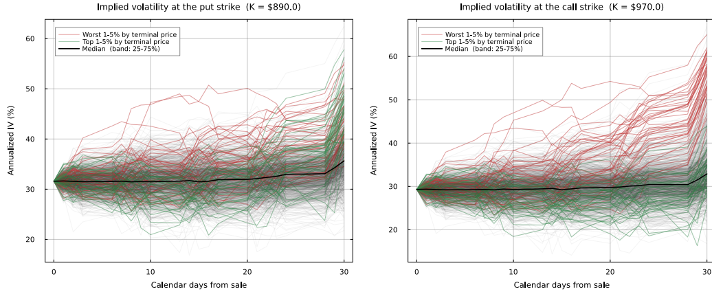
Figure 4: Contract-specific IV paths at the GS put strike (left) and call strike (right). The horizontal axis uses the 31-calendar-day schedule, with values updated on 22 trading transitions. Path colors follow Fig. 3.
