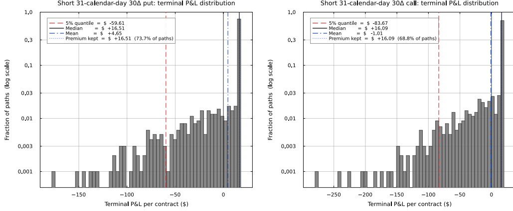
Figure 5: GS terminal short-option P&L per contract over 1,000 JumpHMM paths. The lattice IV process does not enter terminal P&L in (14); it affects only interim values and Greeks.
