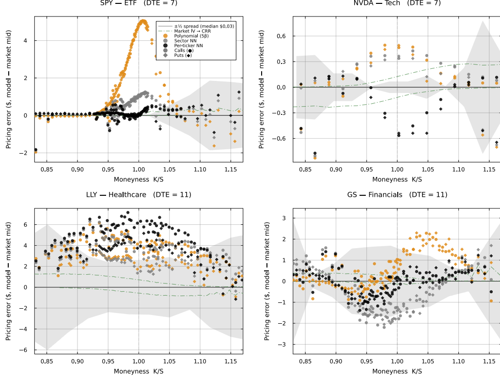
Figure 2: CRR American price minus market mid on May 11, 2026, for SPY, NVDA, LLY, and GS. Curves show the parametric, sector, per-ticker, and market-IV reference inputs. The gray ribbon is the median local bid-ask half-spread by moneyiness bin. A point inside the ribbon has an absolute pricing error below that local half-spread.
