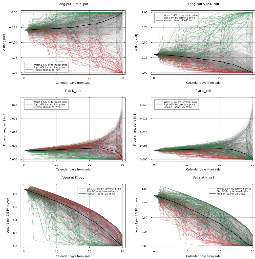
Figure S4: LLY long-option delta, gamma, and Vega from the 201-step Leisen-Reimer pricer. Short-position Greeks have the opposite sign.
