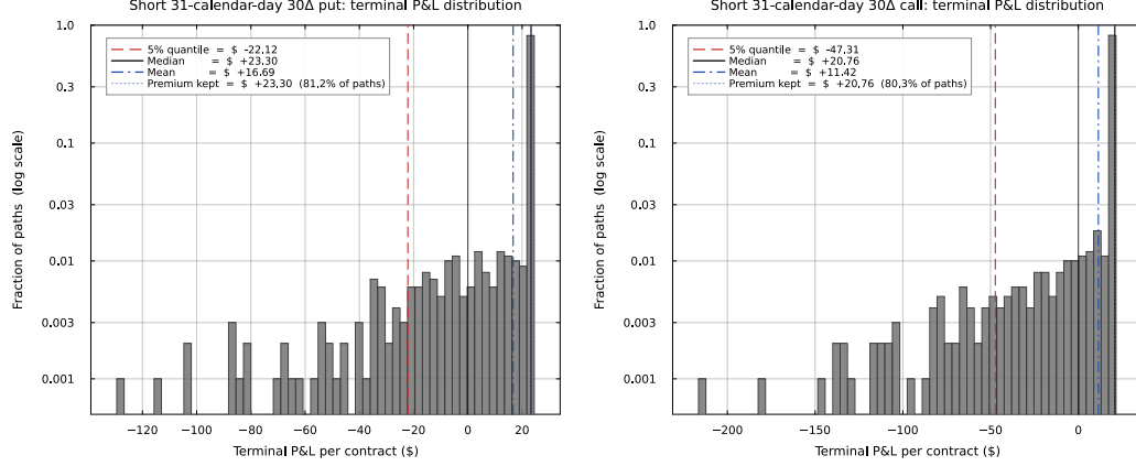
Figure 6: LLY terminal short-option P&L per contract over 1,000 JumpHMM paths. The wider lower tail for the call came from the simulated terminal-stock distribution relative to the call strike and entry premium.
