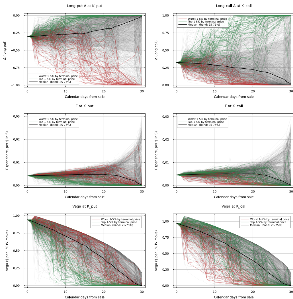
Figure S1: GS long-option delta, gamma, and Vega from the 201-step Leisen-Reimer pricer. Spot bumps were 1.5% of spot, and IV bumps were 0.005. Vega is dollars per one volatility percentage point.
