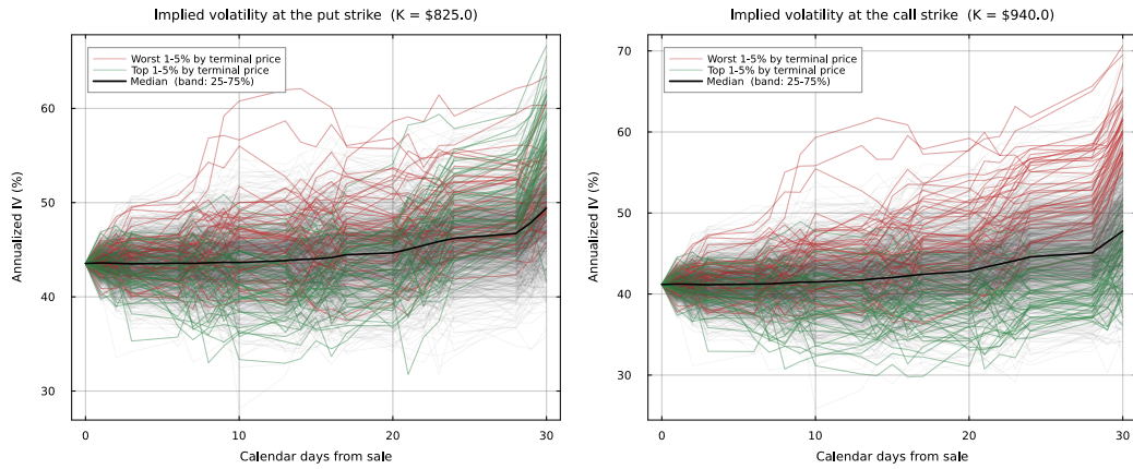
Figure S3: Contract-specific LLY IV paths at the put and call strikes. The fixed negative return-shock coupling tended to raise factor shocks after lower standardized returns.
