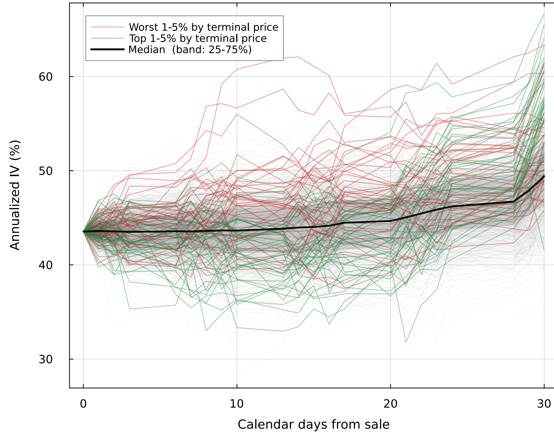
Implied volatility at the put strike (K = $825.0)
