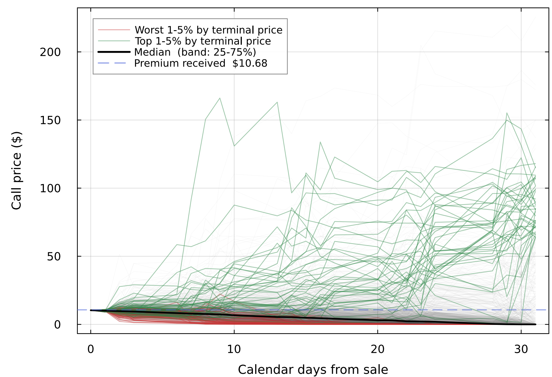
Short 31-calendar-day 30Δ call: option price
