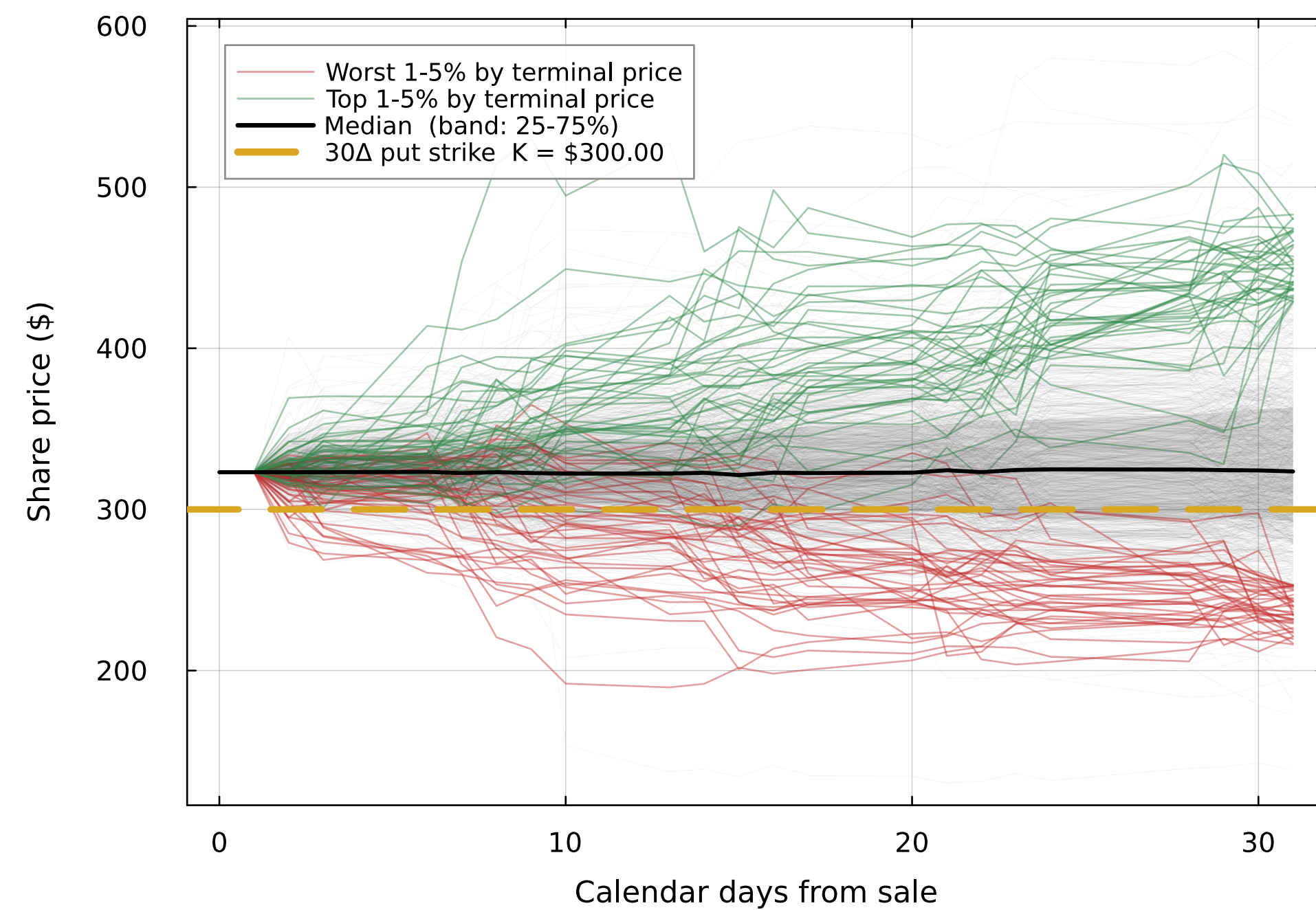
AMD share price paths ( S_0 = \$323.08 )
